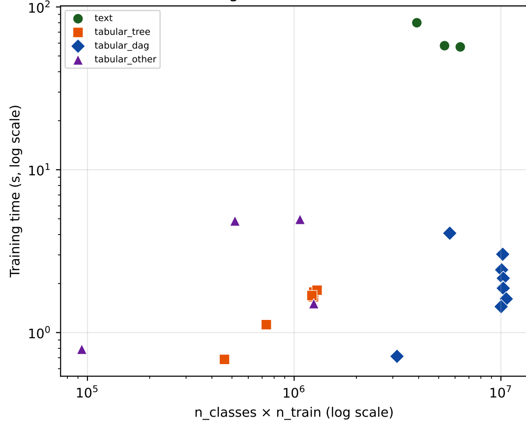
Training Time vs Problem Size
