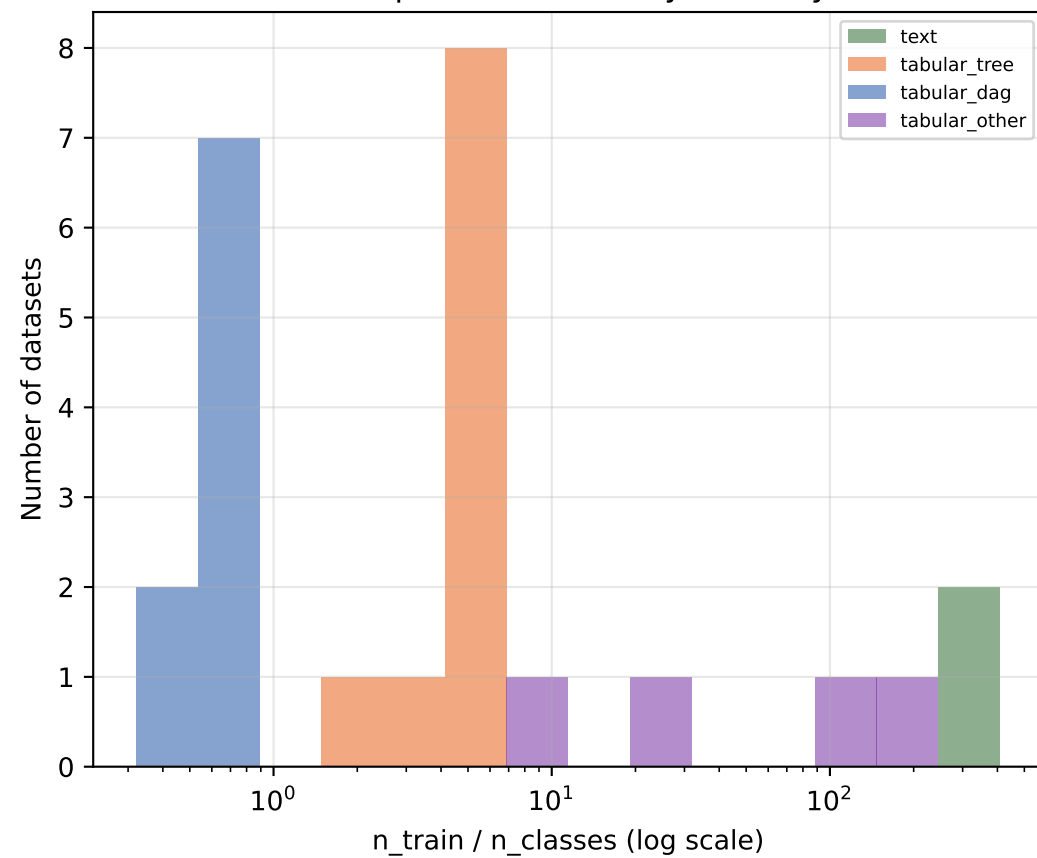
Data-per-Class Ratio by Modality
