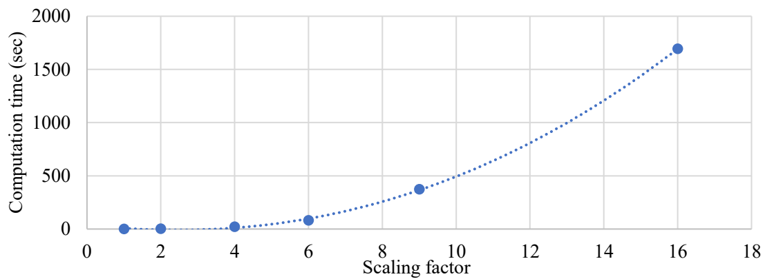
Figure 14. Computation time curve of the SGP algorithm
