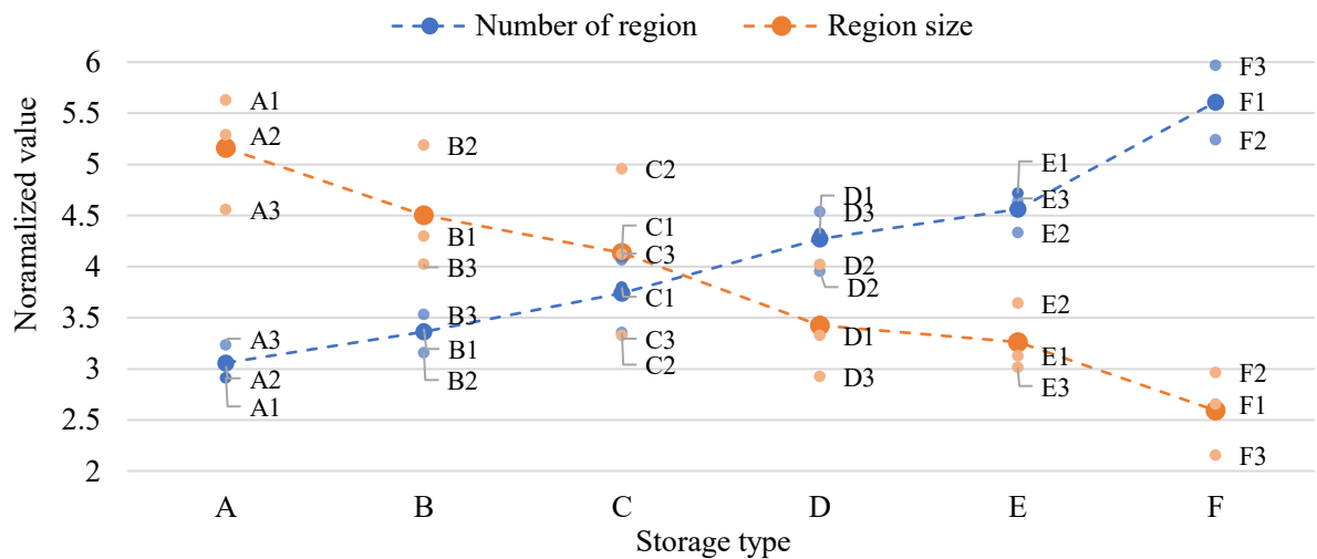
Figure 9. Effect of yard size on region characteristics
