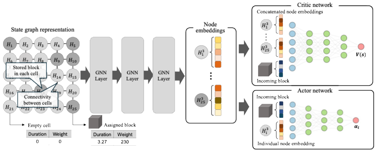
Figure 8. Network structure of graph reinforcement learning for placement algorithm
