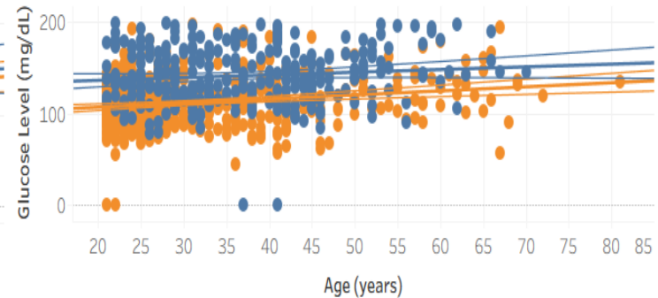
Age vs Glucose Level by Diabetes Status
