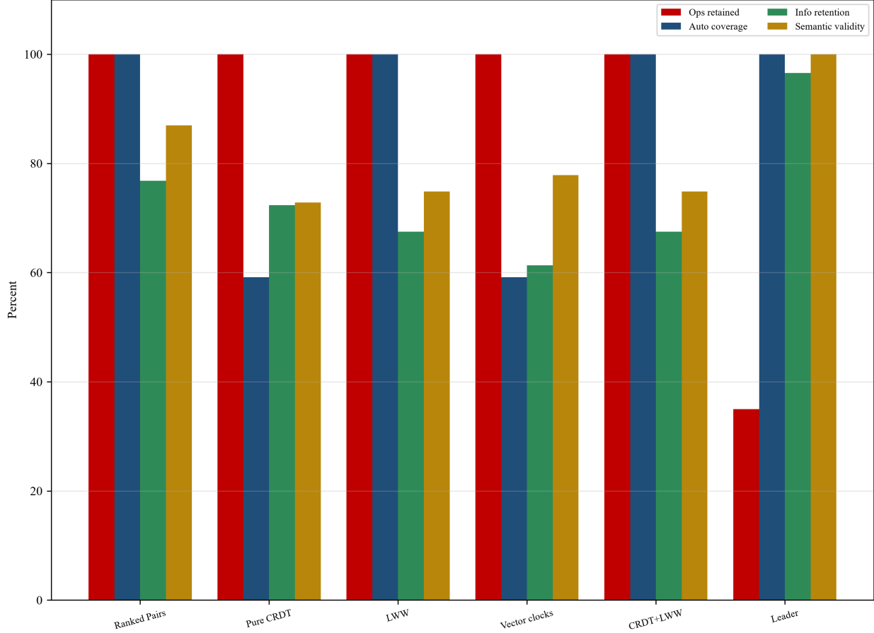
Figure 3: Fig. 3. End-to-end quality at high conflict under partial ballots (no dissemination). Each design decision materializes as a quantified cost on the four axes: leader overwrite retains 35.0% of operations; LWW keeps 67.5% of ordering information and violates 14.4 causal constraints on average; vector clocks automate 59.2% of resolutions and keep 61.3%; pure CRDT covers 59.2%; CRDT+LWW fallback covers everything at LWW quality; CF-RP retains 76.8% of ordering information with zero causal violations and full automation.
