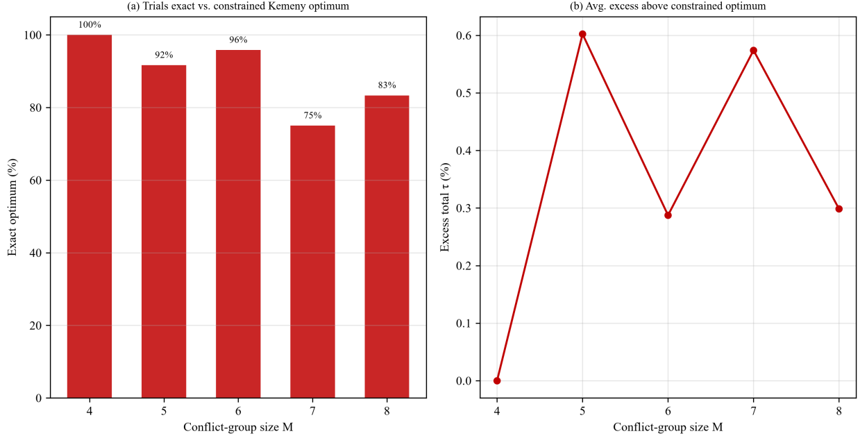
Figure 1: Fig. 1. Validation that \tau -optimal feasible merging is achievable, via its concrete instantiation—the lexicographic (infinite-weight) case of weighted Ranked Pairs (causal edges locked first)—against the causally constrained Kemeny-Young optimum at small conflict-group sizes ( N = 10 , 24 trials each, partial ballots, no dissemination). (a) Fraction of trials in which the instantiation achieves the exact constrained optimum. (b) Excess total \tau distance above the constrained optimum. The instantiation is exact in 89% of trials overall, with average excess 0.35% (maximum 8.0% in a single M = 5 trial); the constrained and unconstrained optima coincide in 100% of these trials.
