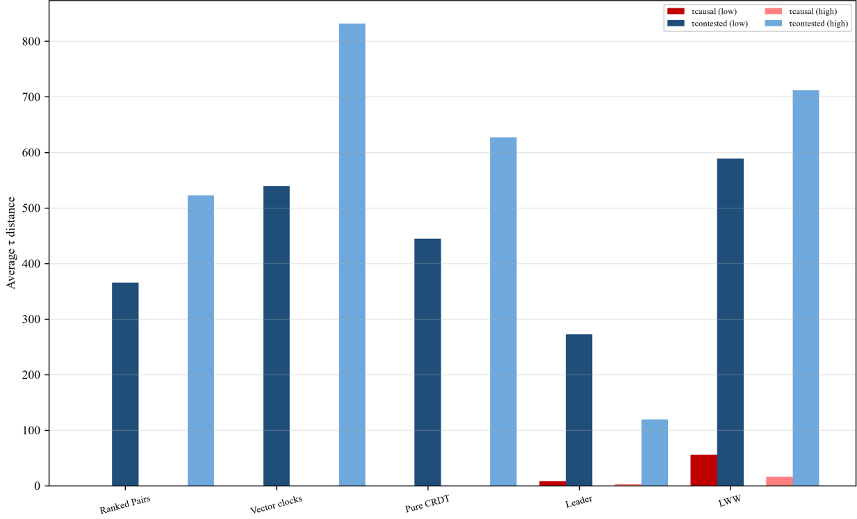
Figure 2: Fig. 2. Causal decomposition of total \tau distance (Proposition 2) on partial ballots without dissemination. Red: \tau_{\text{causal}} (causal-constraint violations). Blue: \tau_{\text{contested}} (genuine ordering disagreement). Dark bars: low conflict (35% causal density). Light bars: high conflict (10% causal density). \tau_{\text{causal}} is identically zero for CF-RP, vector clocks, and pure CRDT at both conflict levels—the constraint holds by construction—while timestamp-based LWW and CRDT+LWW incur 16.2 (high) to 55.3 (low) causal violations per trial on average, which the metric counts exactly; leader overwrite’s timestamp-append fallback incurs 2.7–8.3.
