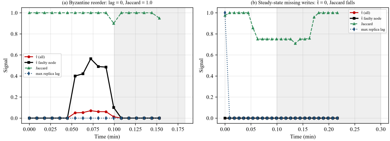
Figure 7: Fig. 7. Fault-injection monitoring on the Cassandra cluster (E7). (a) Byzantine reorder: \hat{\tau} rises and the faulty replica’s per-node \hat{\tau} dominates while lag \equiv 0 and Jaccard \equiv 1.0 . (b) Steady-state missing writes: \hat{\tau} \equiv 0 while Jaccard falls—set-level faults are invisible to \tau and caught by the Jaccard/repair signals. Shaded region: fault window.
