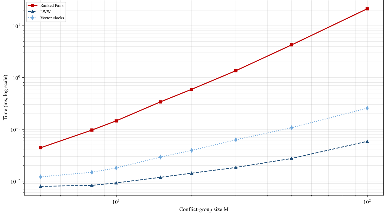
Figure 6: Fig. 6. Reconciliation time versus conflict-group size (log scale) on partial ballots. CF-RP is sub-millisecond for typical groups ( M \leq 20 ), 1.35 ms at M = 30 , 4.4 ms at M = 50 , and \approx 21 ms at M = 100 —an extreme case; causal pre-locking adds no measurable overhead over plain Ranked Pairs. LWW and VC detection are cheaper but produce the quality losses measured above.
