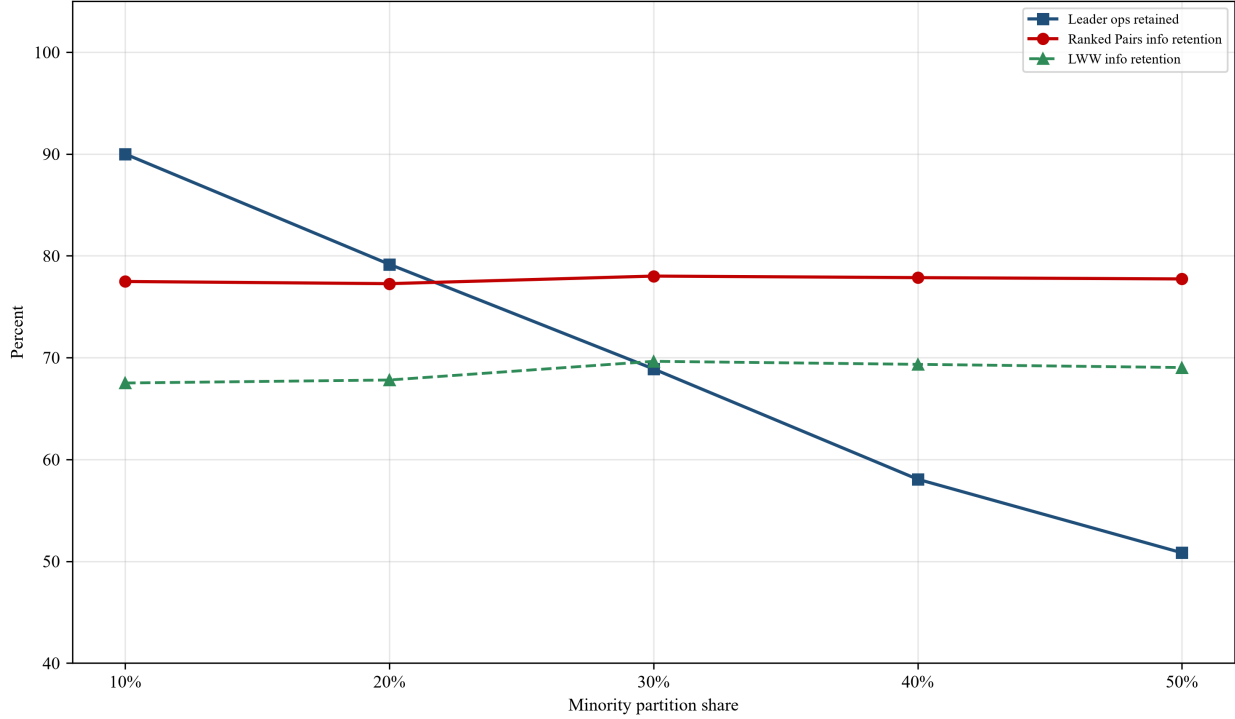
Figure 5: Fig. 5. As the minority partition grows, leader-based overwrite retains fewer operations (90% \rightarrow 51%). Full-retention strategies (LWW, CF-RP) stay flat on ordering information retention, with CF-RP consistently 8–10 percentage points above LWW.
