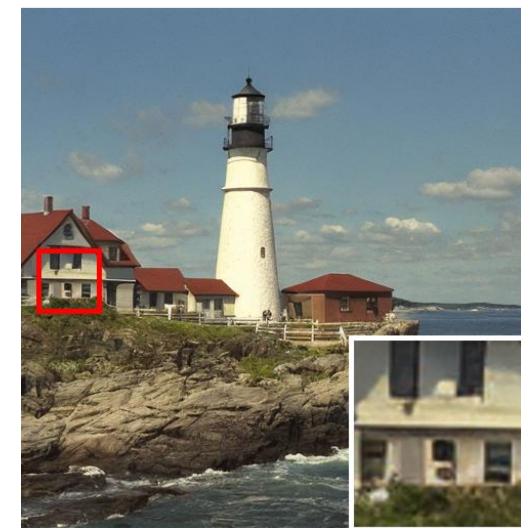
OSCAR
