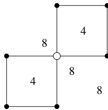
FIGURE 1. Two quadrilaterals sharing the white cut vertex. The numbers indicate face sizes; the unbounded face is written at each of the three corners it occupies, two of them at the white vertex, which the exterior boundary walk therefore encounters twice. Its length is 8, the number of edge-side incidences it carries, although only 7 distinct vertices lie on it. This is a convention example, not an alternating plane graph.
