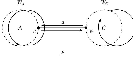
FIGURE 4. The dashed outlines represent the components A and C of G - a , with their internal edges omitted; W_A and W_C are their exposed facial walks, which need not be cycles. The face F carrying the bridge a = uw follows W_A , crosses a , follows W_C , and crosses a again in the opposite direction — the two arrows along a are two traversals of one edge, not two edges. Hence |F| = |W_A| + |W_C| + 2 , and under the hypotheses of Lemma 5.1 both walks have length at least 3, so |F| \geq 8 .
