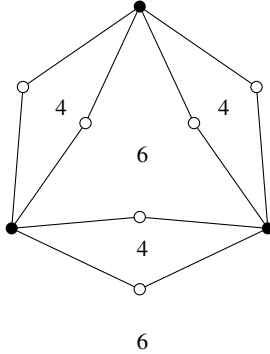
FIGURE 2. The graph of Example 3.2: 9 vertices, 12 edges, 5 faces. Filled vertices have degree 4; white vertices have degree 2, violating the minimum degree 3 required of an alternating plane graph. Face sizes are shown inside the faces, the unbounded face having size 6. Every edge joins a degree-2 vertex to a degree-4 vertex and separates a 4-face from a 6-face, so c(a) = \frac{1}{2} + \frac{1}{4} + \frac{1}{4} + \frac{1}{6} = \frac{7}{6} on all 12 edges.
