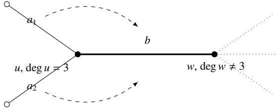
FIGURE 5. The assignment at the degree-3 end u of an eligible edge. Parity forces u to lie on exactly one bridge b = uw , leaving exactly two non-bridge edges a_1, a_2 at u , both assigned to b (dashed arrows, which are assignments and not edges of the graph). Alternation forbids \deg w = 3 , so b receives nothing through w ; the further edges at w are dotted. This is a local configuration in a hypothetical counterexample, not a graph in its own right.
