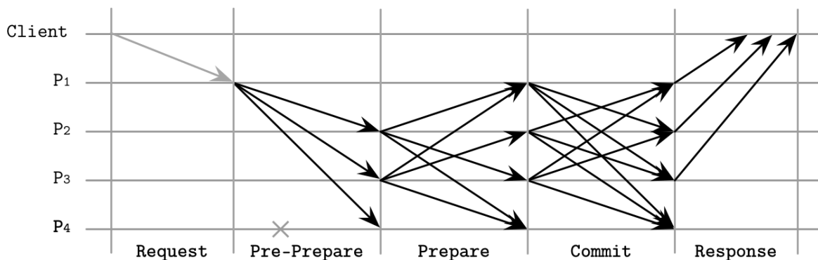
Figure 14-13. PBFT consensus, normal-case operation
