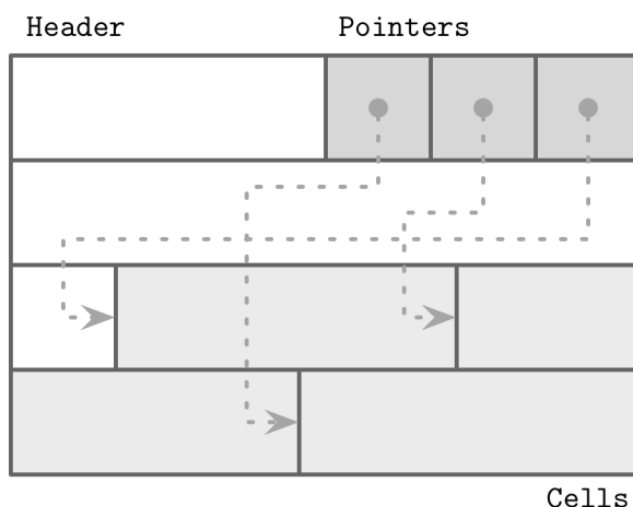
Figure 3-5. Slotted page
