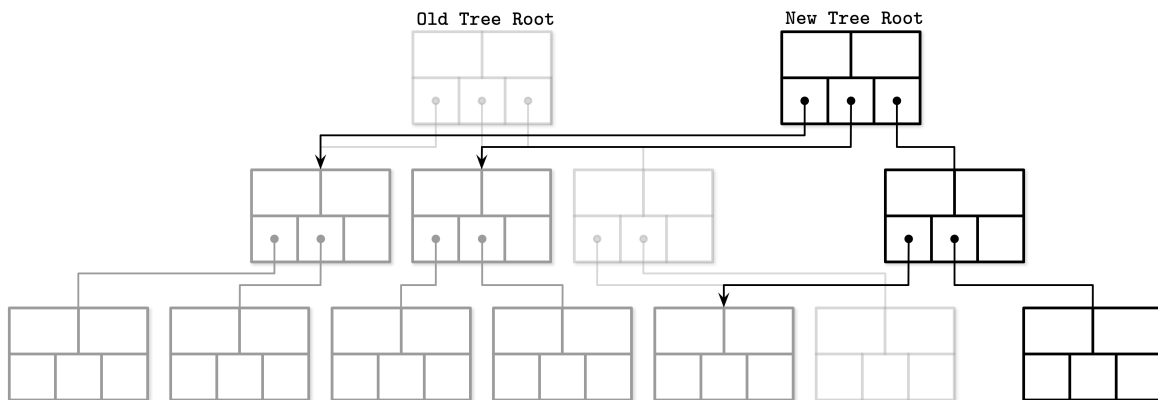
Figure 6-1. Copy-on-write B-Trees
