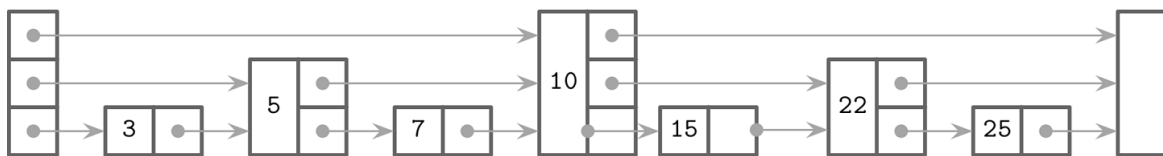
Figure 7-8. Skiplist
