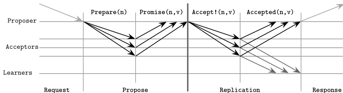
Figure 14-3. Paxos algorithm: normal execution
