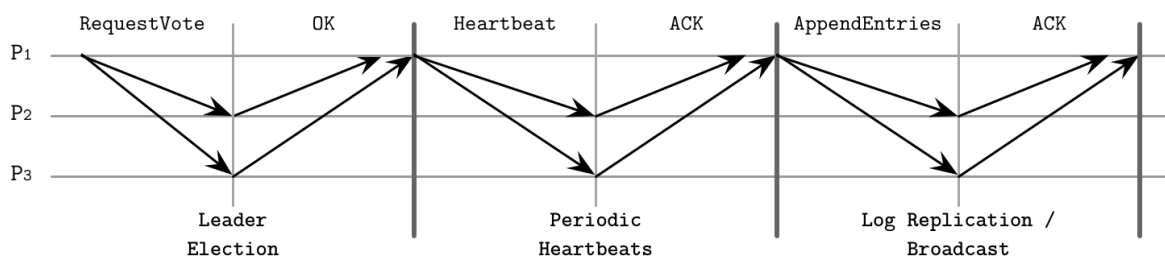
Figure 14-10. Raft consensus algorithm summary
