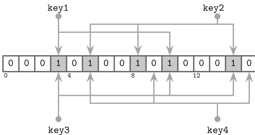
Figure 7-7. Bloom filter
