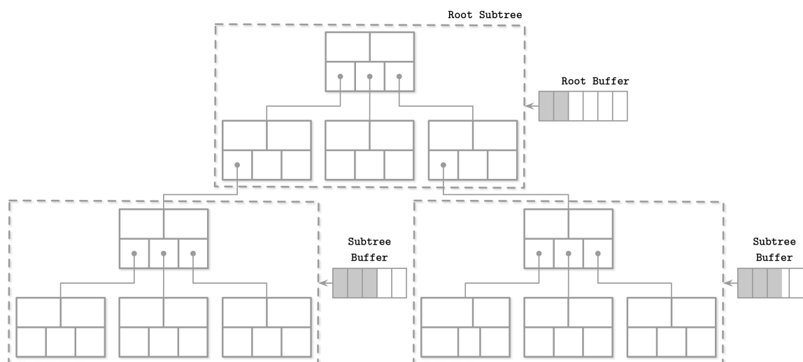
Figure 6-4. LA-Tree
