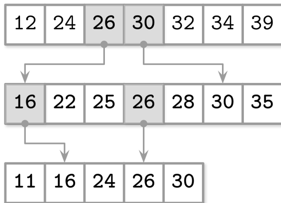
Figure 6-5. Fractional cascading
