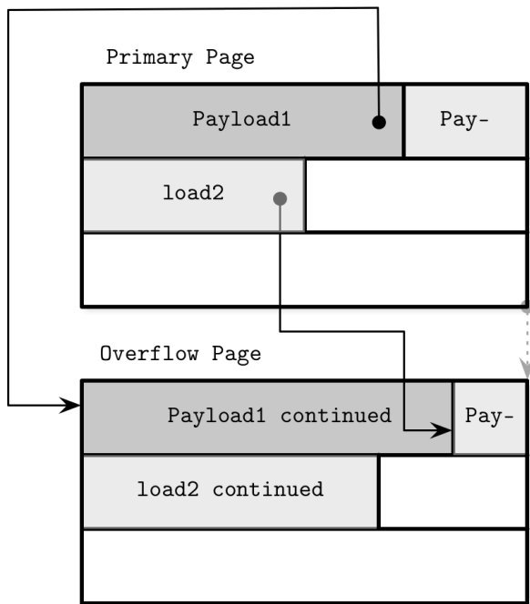
Figure 4-6. Overflow pages
