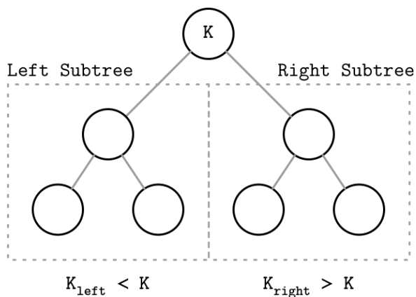
Figure 2-2. Binary tree node invariants
