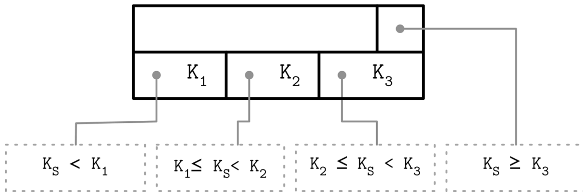
Figure 4-2. Rightmost pointer
