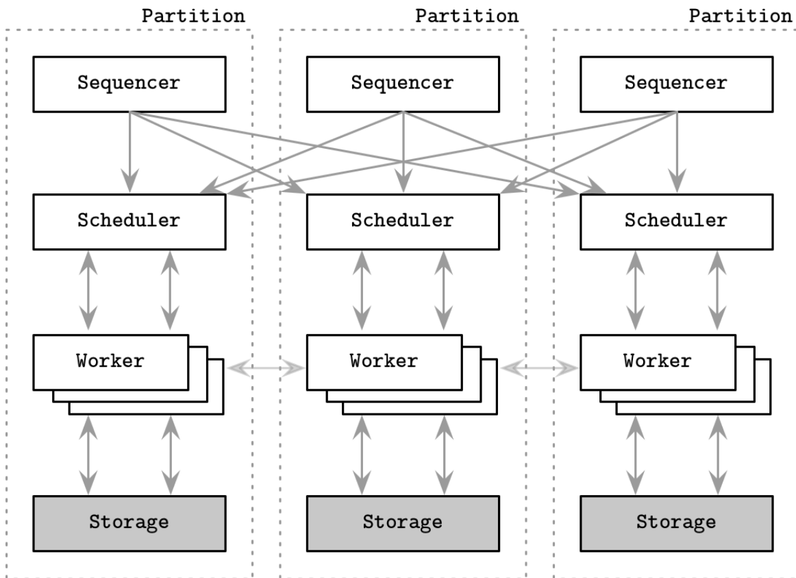
Figure 13-7. Calvin architecture
