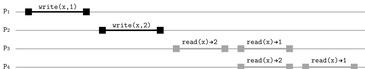
Figure 11-5. Ordering in sequential consistency
