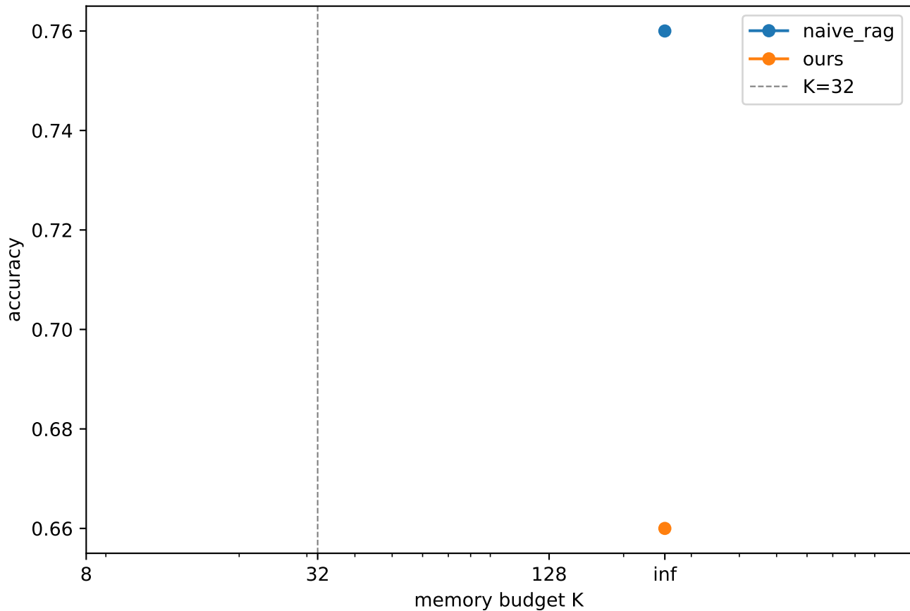
EXP-2: Memory-budget Pareto
