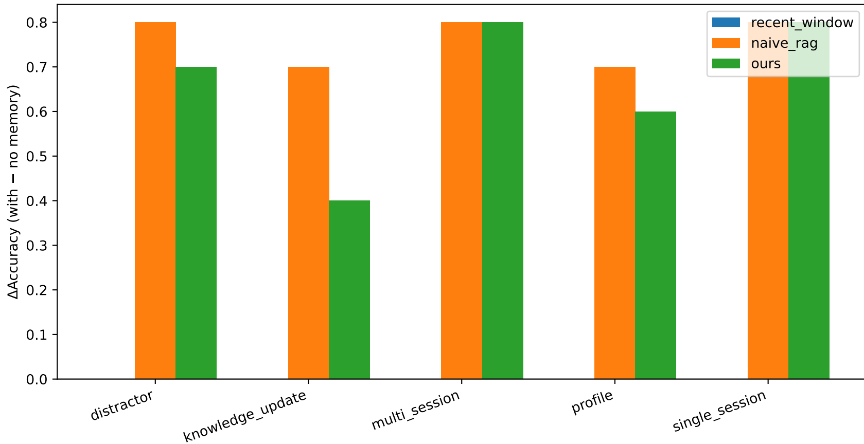
EXP-1: Counterfactual \Delta Accuracy by category
