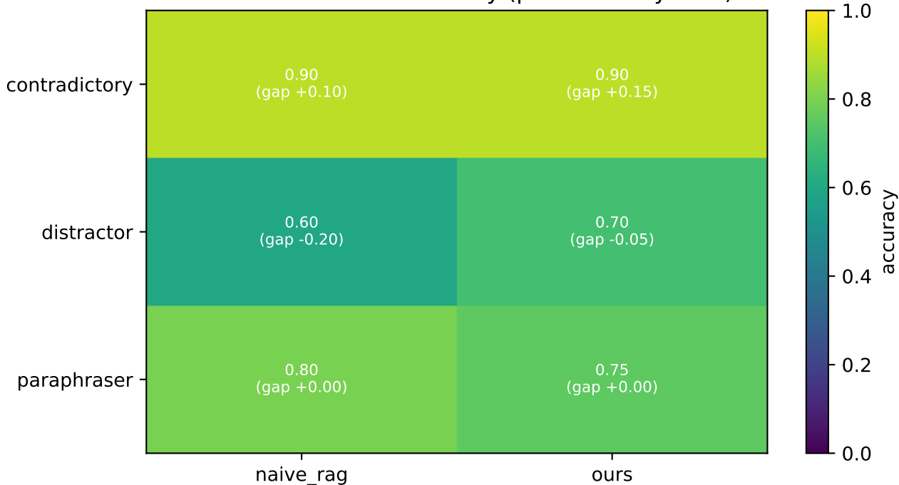
EXP-3: Adversarial accuracy (persona × system)
