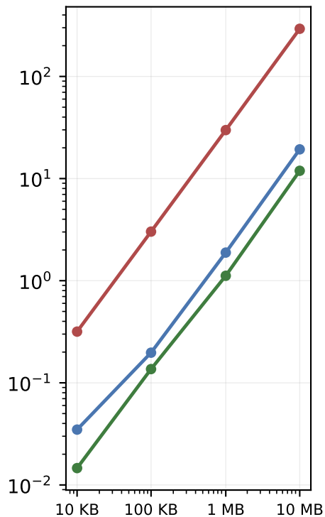
Punkt sentence split
