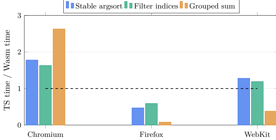
Fig. 6 Browser kernel ratios at 100,000 rows. The dashed parity line exposes the engine-dependent reversal.
