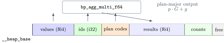
Fig. 2 Wasm linear-memory layout for fused aggregation. The arena begins at the linker-exported heap base; every top-level call copies results before resetting the arena.
