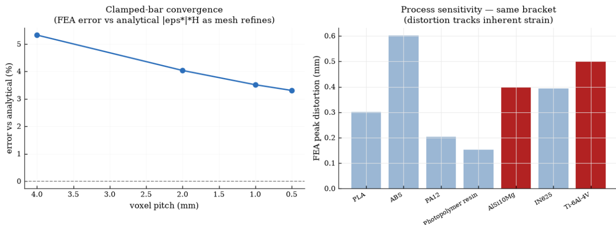
Figure 6: FEA validation
