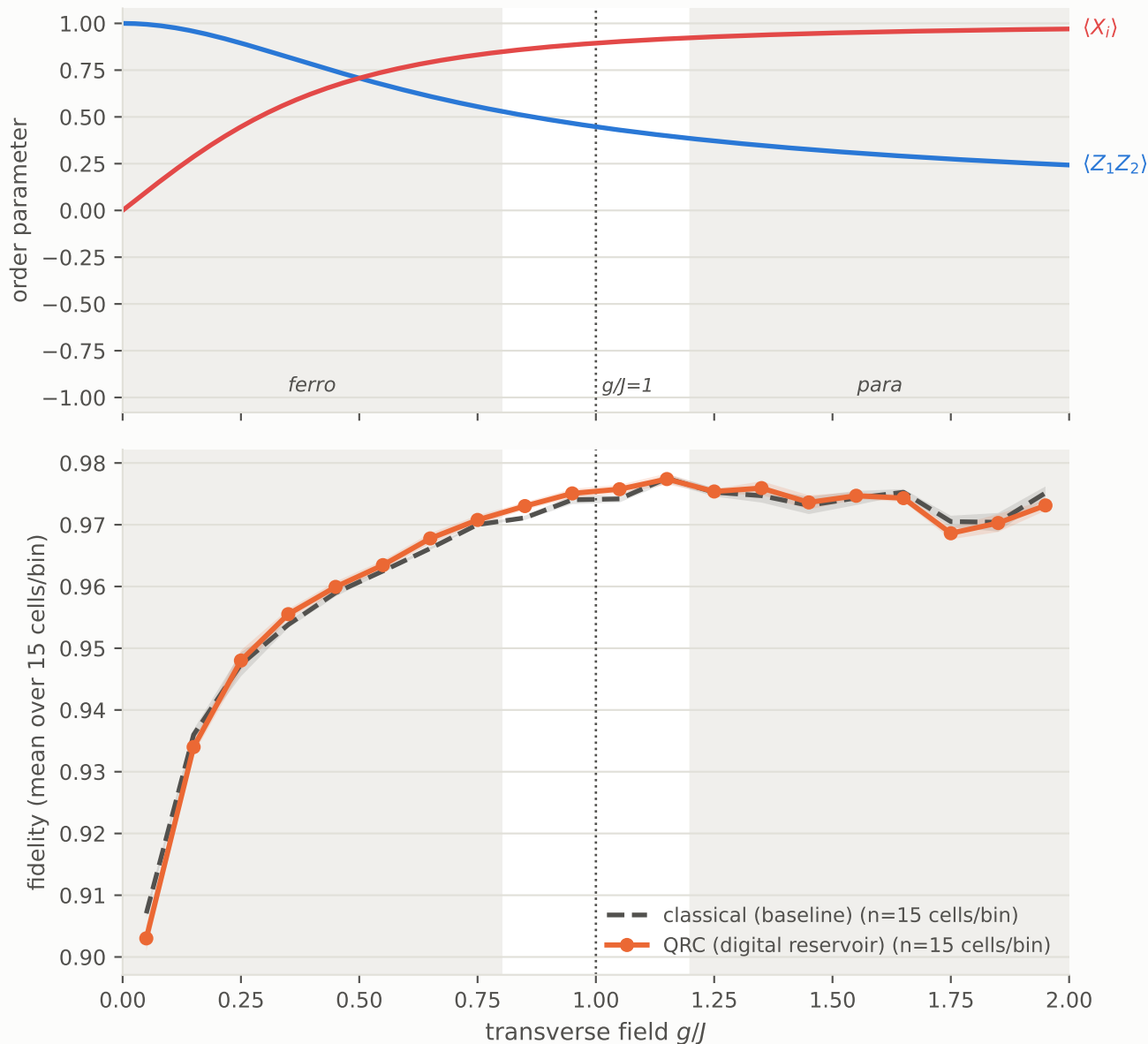
TFIM ground state (N=2): physical phase diagram vs. digital-reservoir (QRC) reconstruction fidelity
