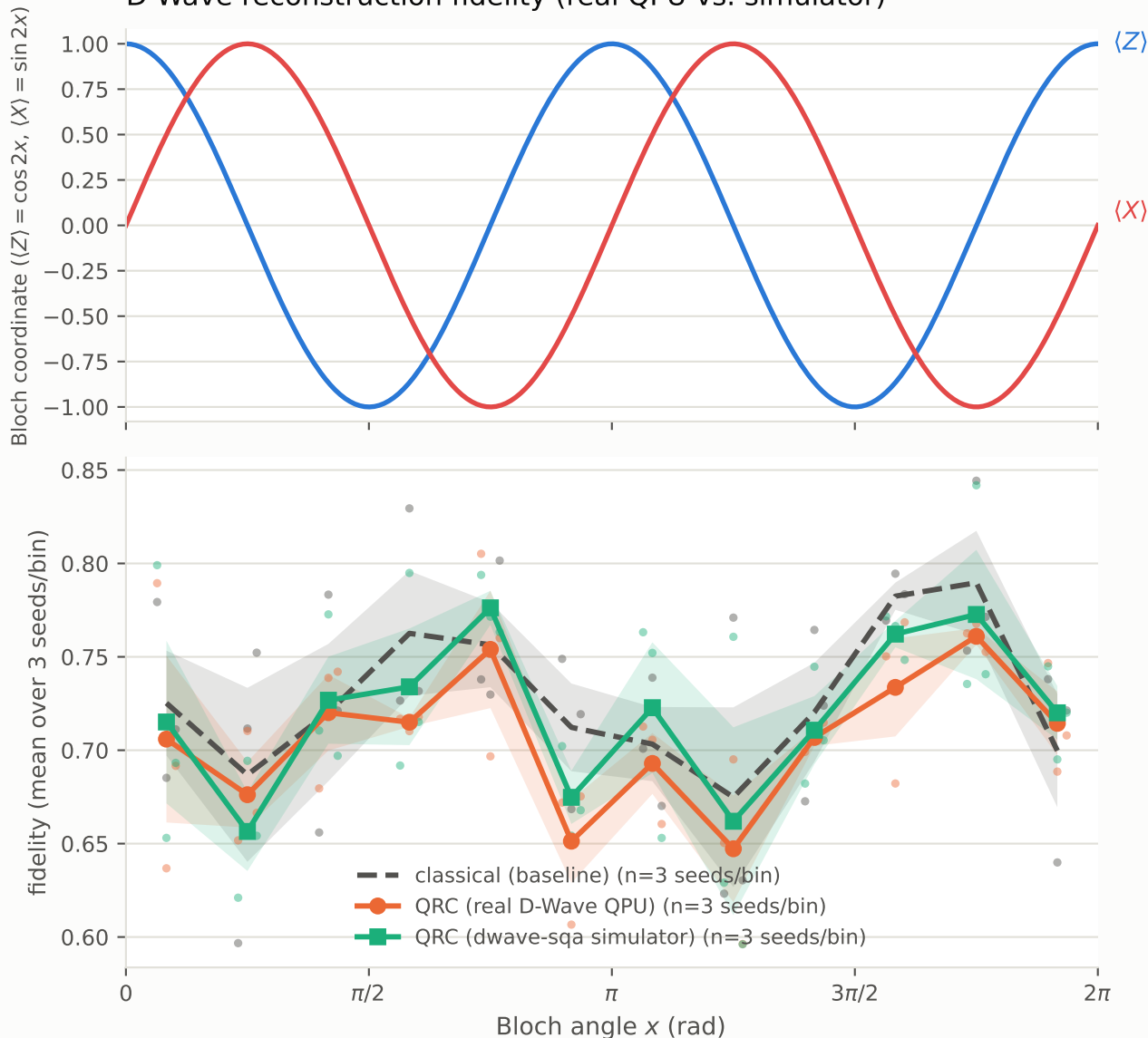
Circular states (N=1): position on the Bloch circle vs. D-Wave reconstruction fidelity (real QPU vs. simulator)
