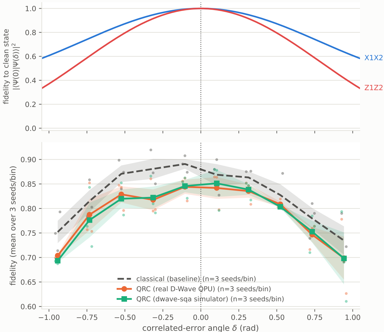
Correlated noise (N=2): distance from clean state vs. D-Wave reconstruction fidelity (real QPU vs. simulator)
