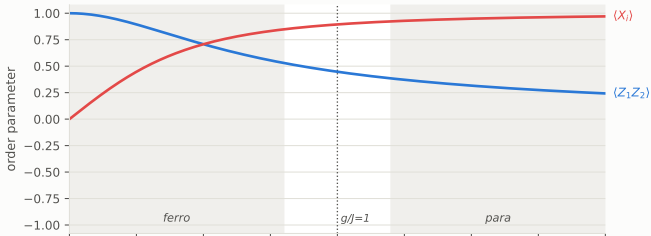
TFIM ground state (N=2): physical phase diagram vs. D-Wave reconstruction fidelity (real QPU vs. simulator)
