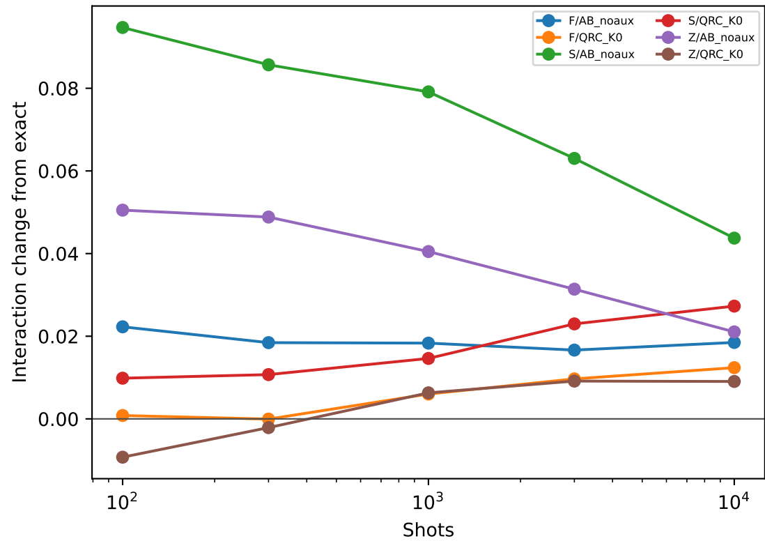
Kernel contrast stability
