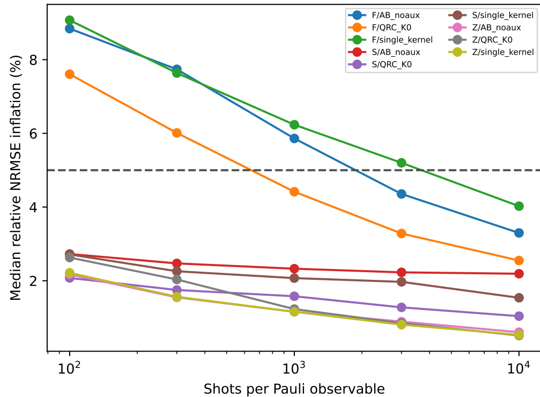
Finite-shot readout sensitivity
