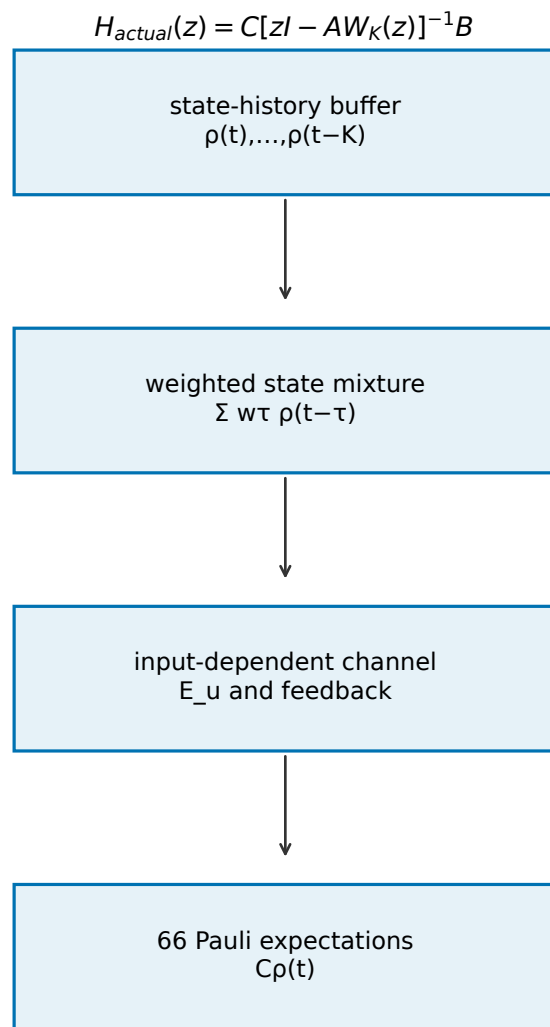
(a) State history inside recurrent feedback
