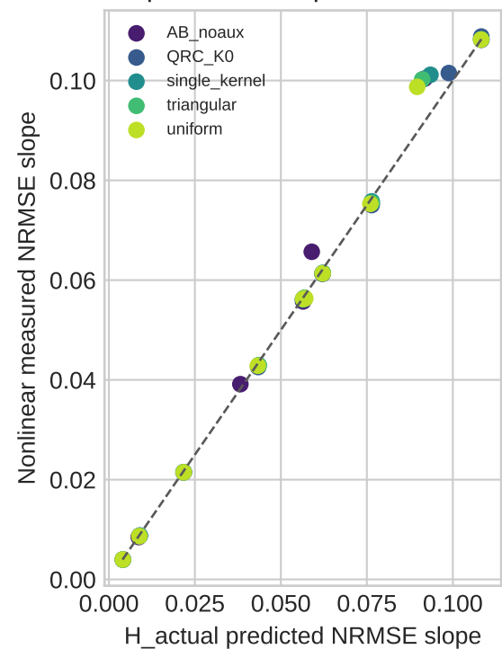
All processes: Spearman=0.99
