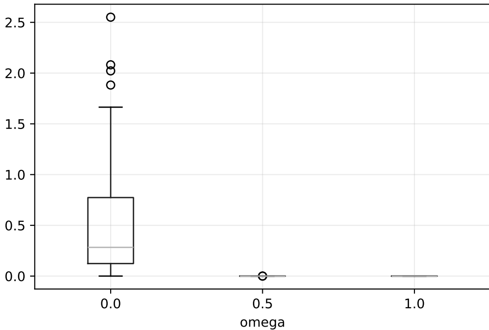
Non-Markovianity by Omega (100 seeds)
