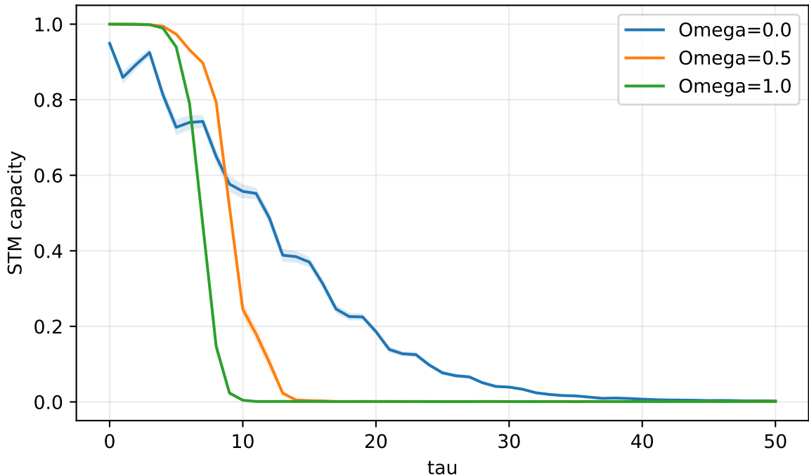
AB embedded STM, 100 seeds, washout/train/test=1000/1000/1000
