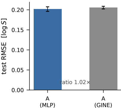
(a) random split
