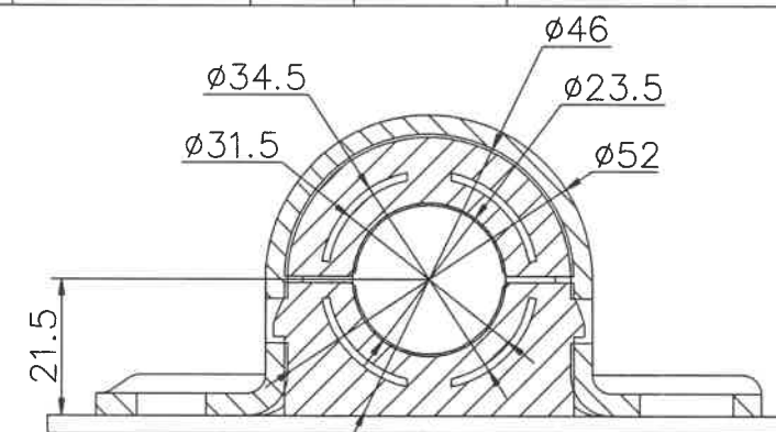
衬套安装状态示意图 Bush Installation Condition Diagram
