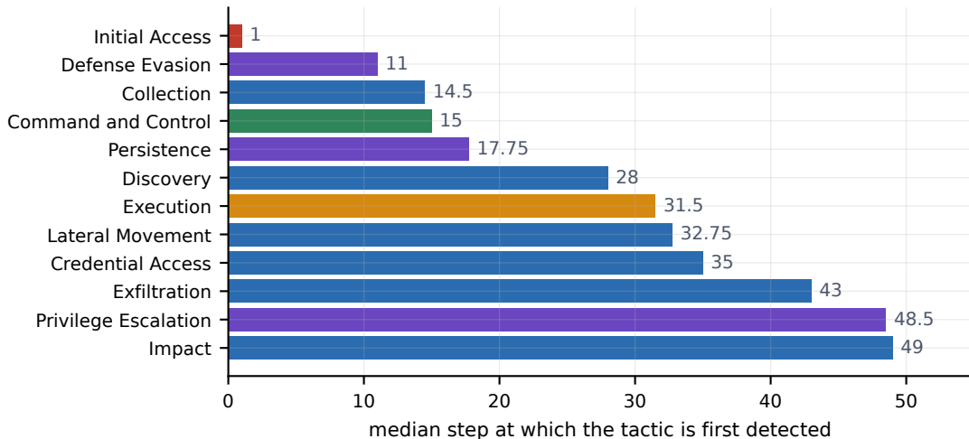
First detection by tactic, 347 campaigns, 45 rules
