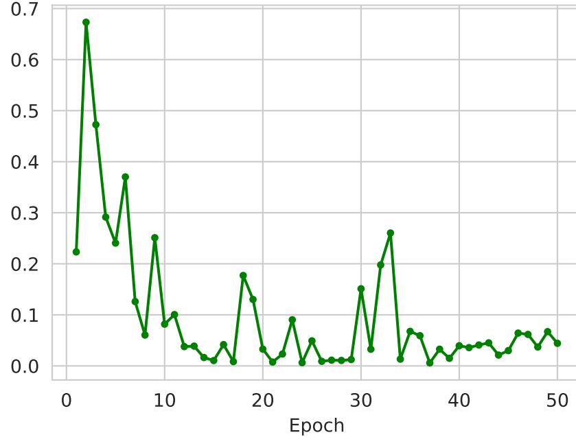
Val Proxy
