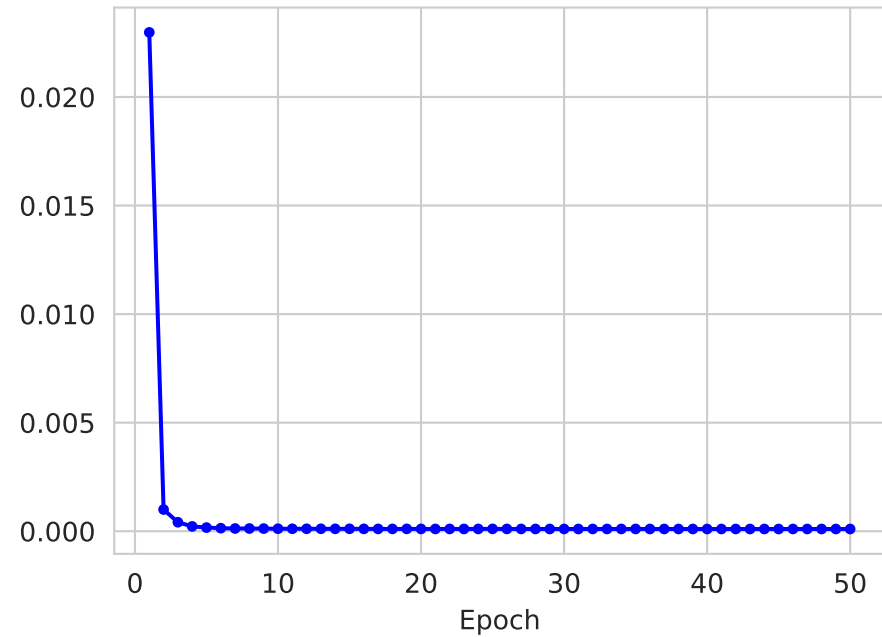
Train Loss
