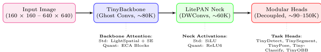
Figure 1: TinyYOLO overall architectural pipeline showing standard vs. quantized configurations.
