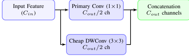
Fig. 2. Architectural details of the GhostConv block.
