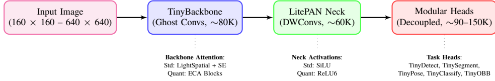
Fig. 1. TinyYOLO overall architectural pipeline showing standard vs. quantized configurations.
