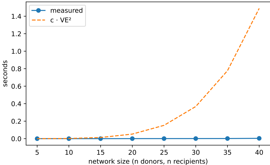
Organ Transplant Network Flow: Runtime vs Size
