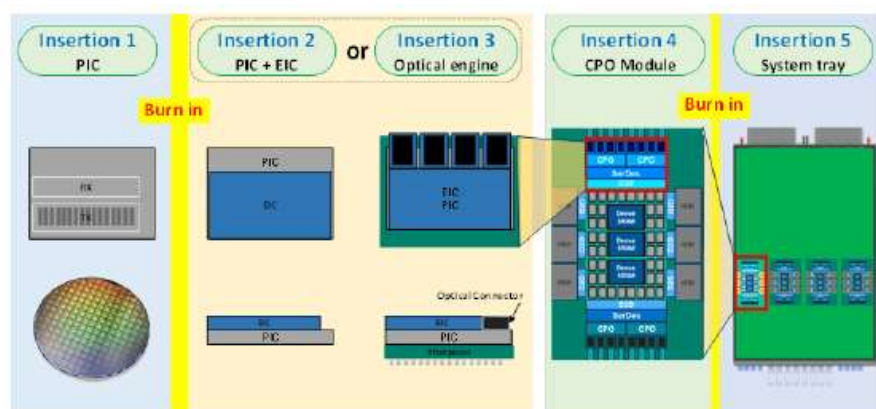
圖三：CPO Test Insertions
