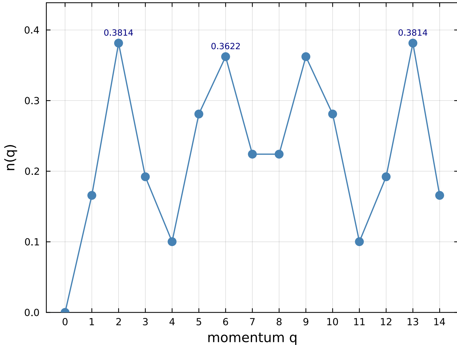
Tilted 30-site ( 4 \times 4 - 1 ), N_p=5 : Structure Factor n(q) [glob t=1, t'=0.2, V_1=1, V_2=V_3=0
