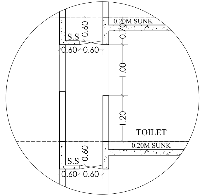
SECTION THROUGH TOILET DUCT DETAIL A-A SCALE 1:50
