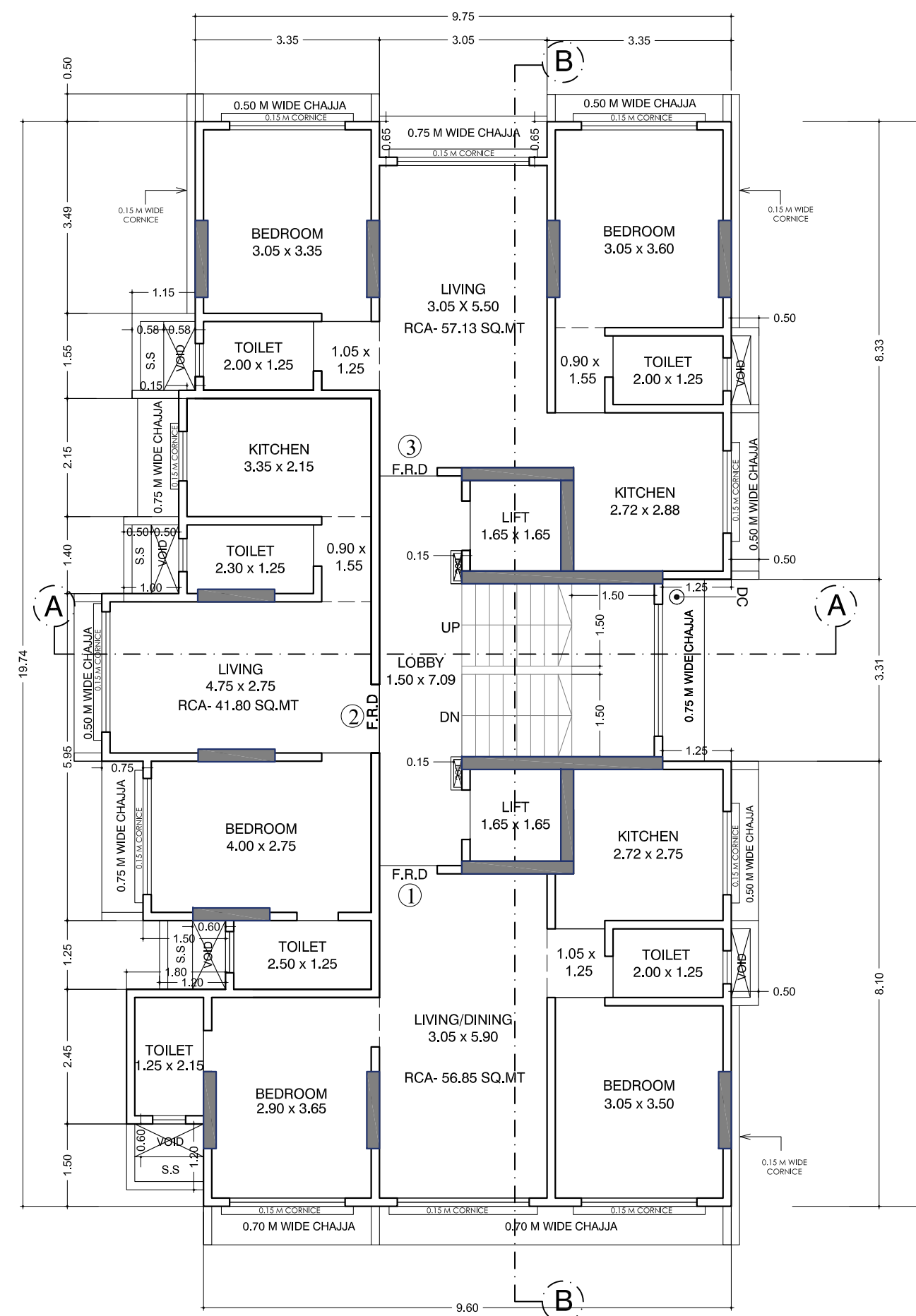
5TH TO 9TH FLOOR PLAN
