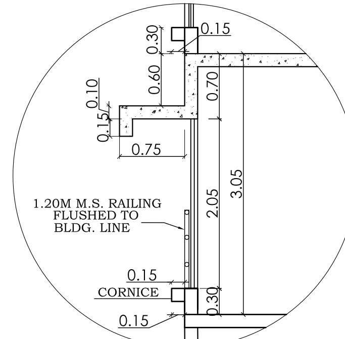
DETAILS OF B-B SCALE - 1:50
