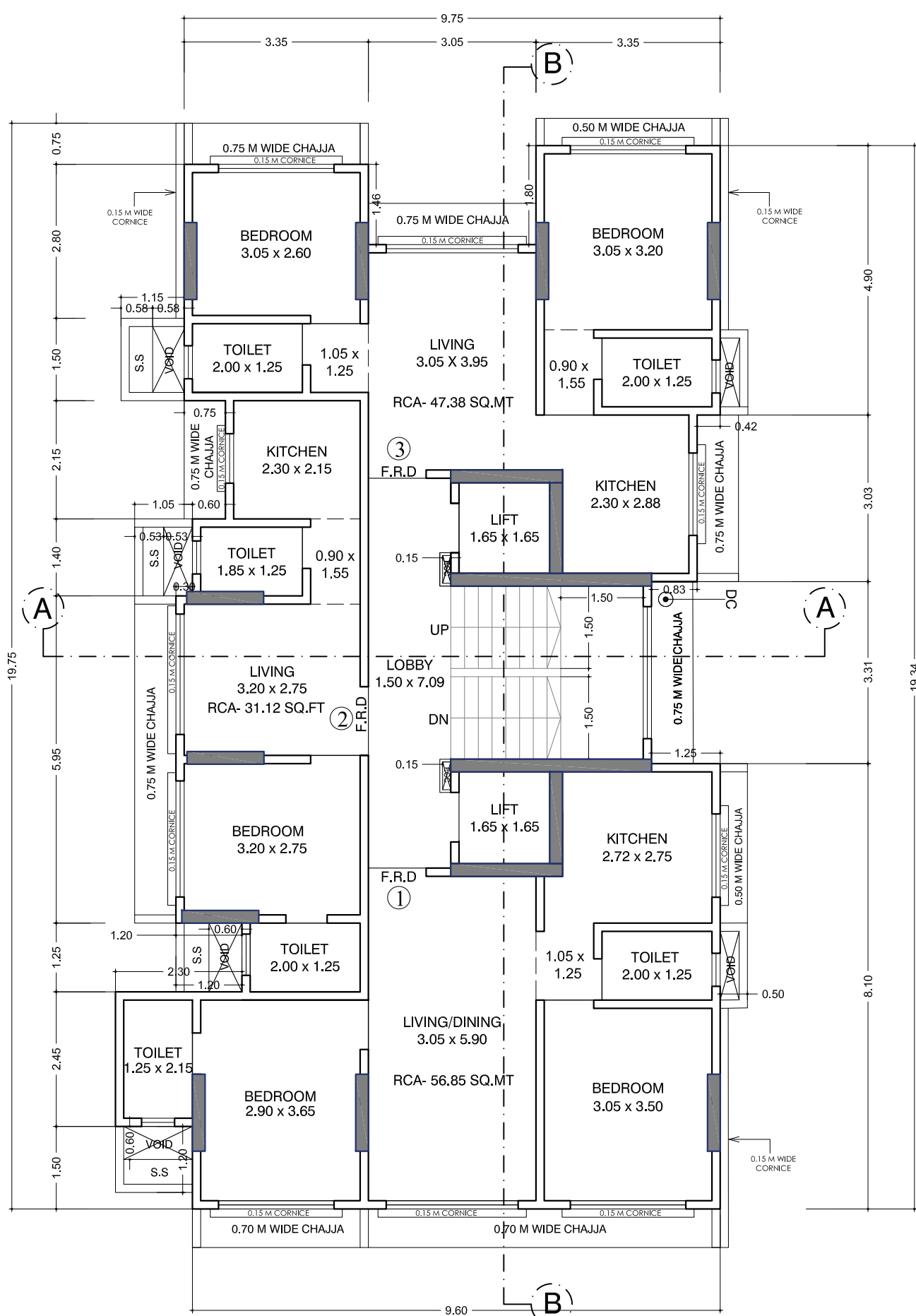
1ST - 3RD FLOOR PLAN
