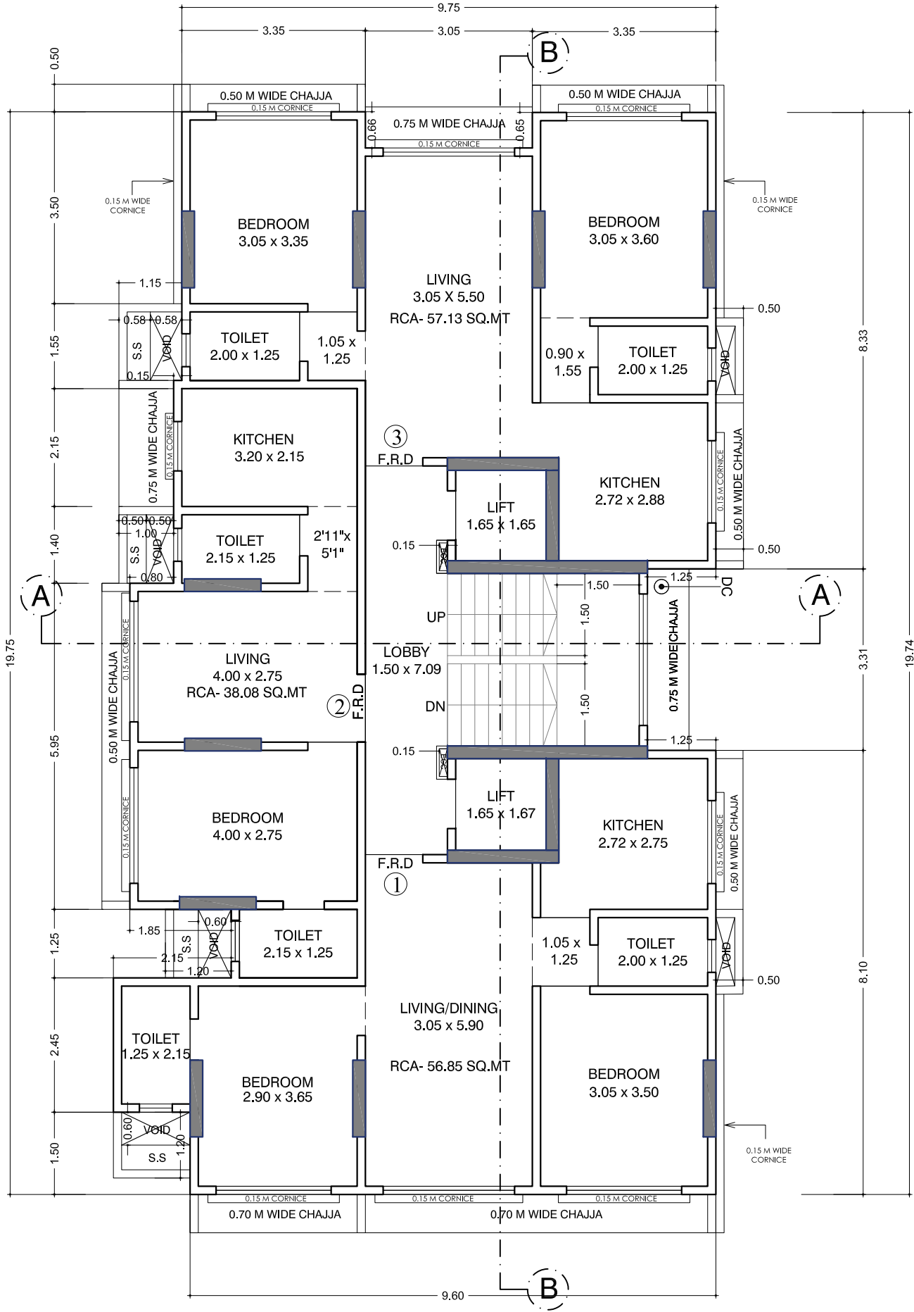
4TH FLOOR PLAN
