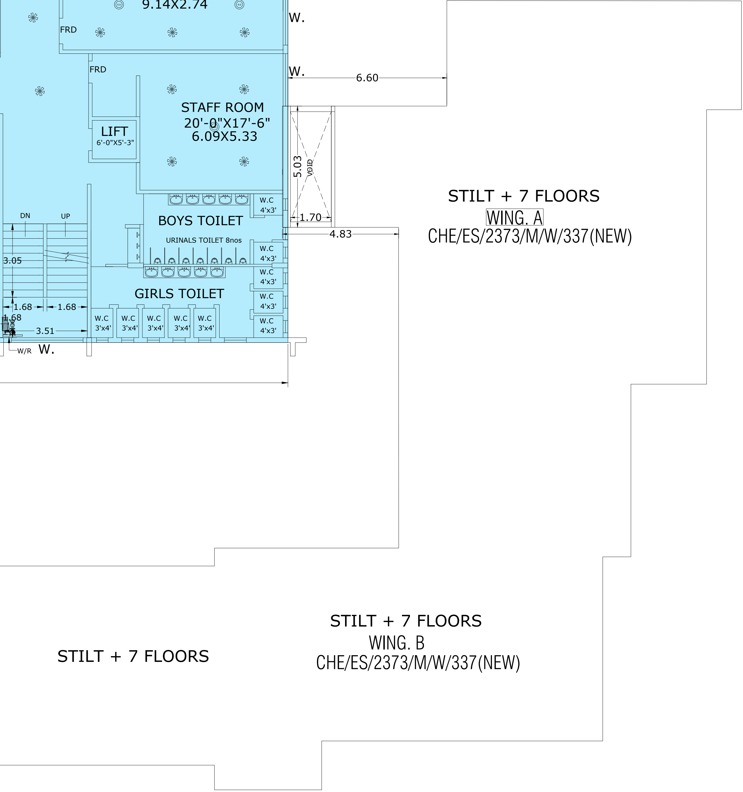
SECOND FLOOR PLAN SCALE :- 1:100
