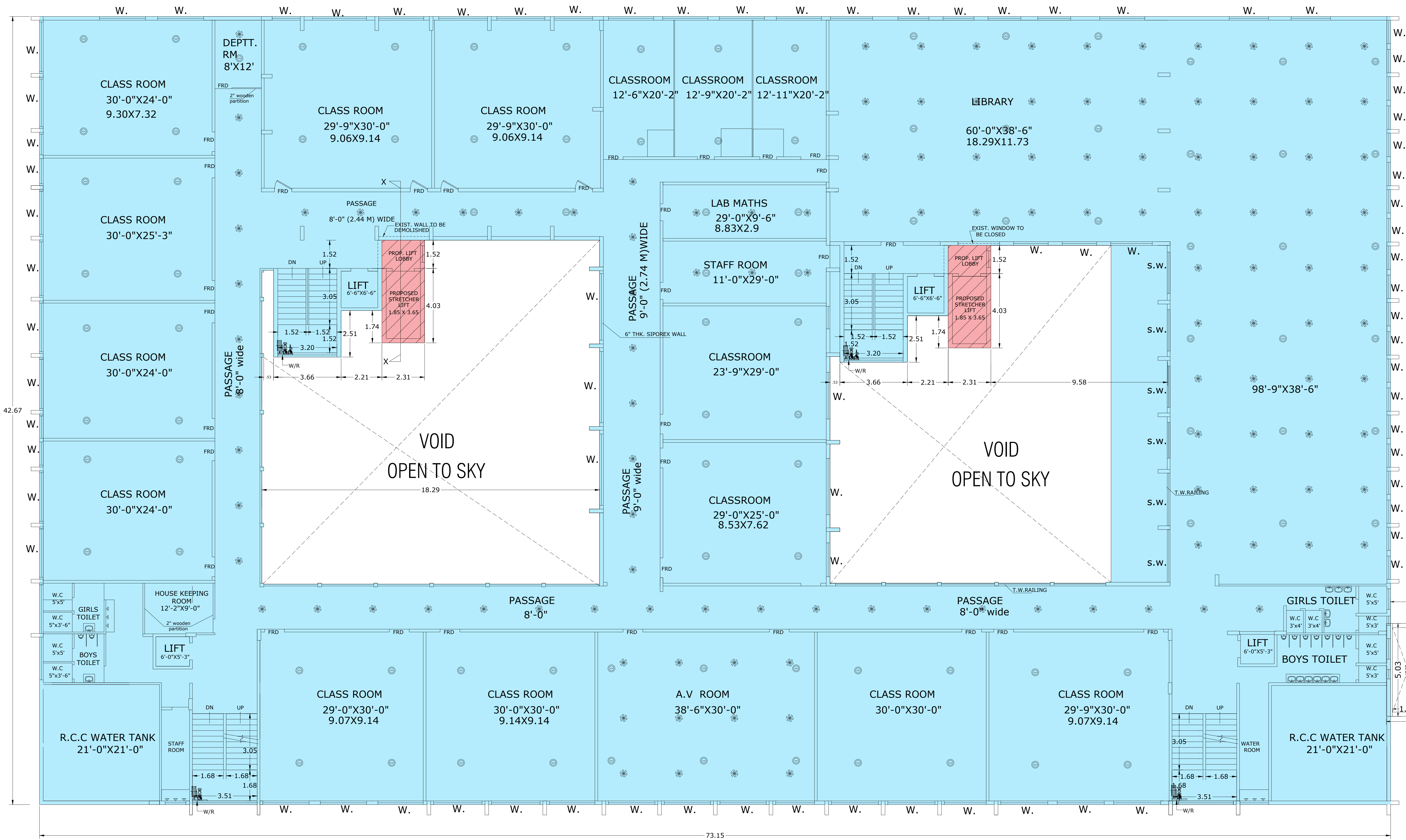
EXISTING FOURTH FLOOR PLAN SCALE : 1:100
