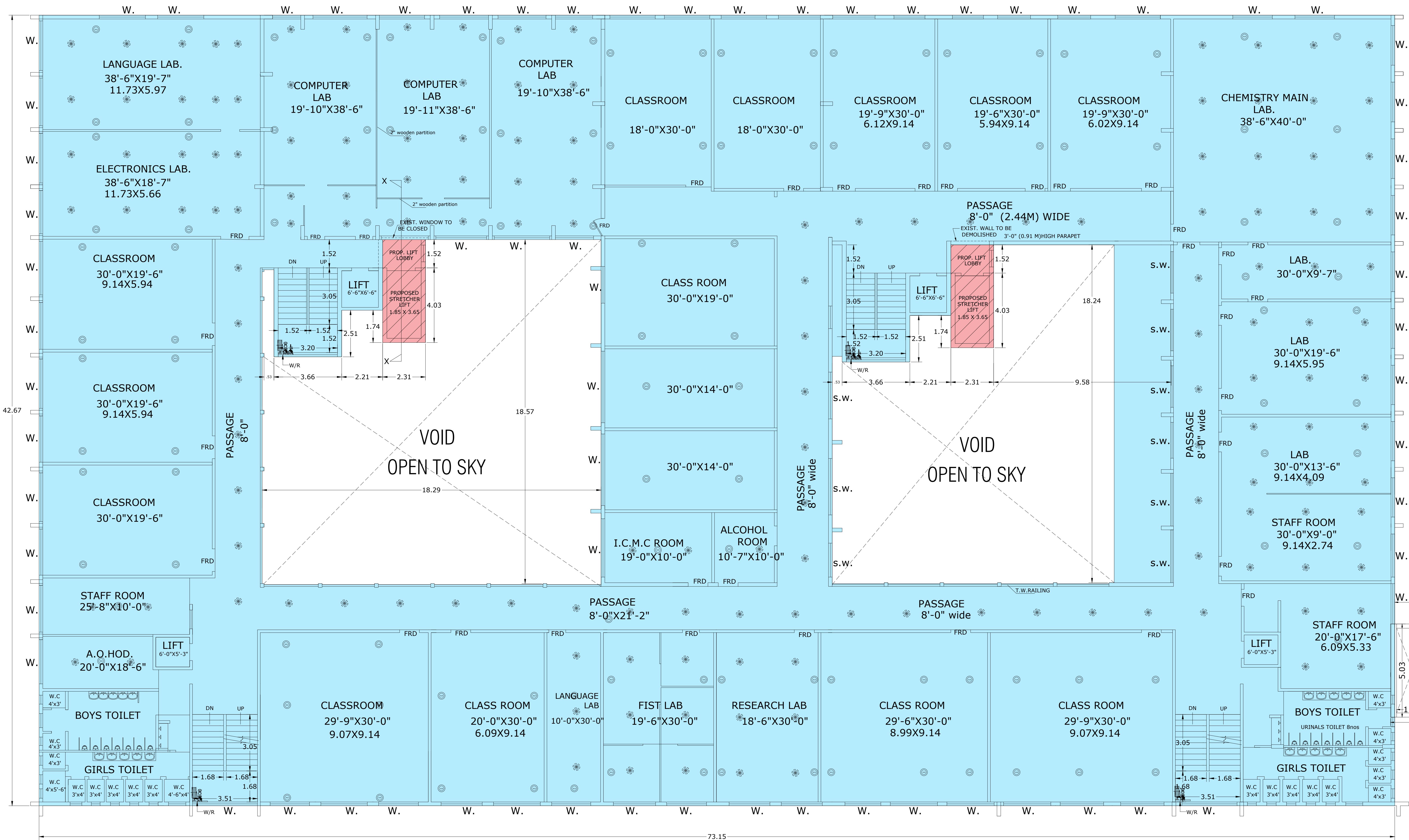
EXISTING SECOND FLOOR PLAN SCALE : 1:100
