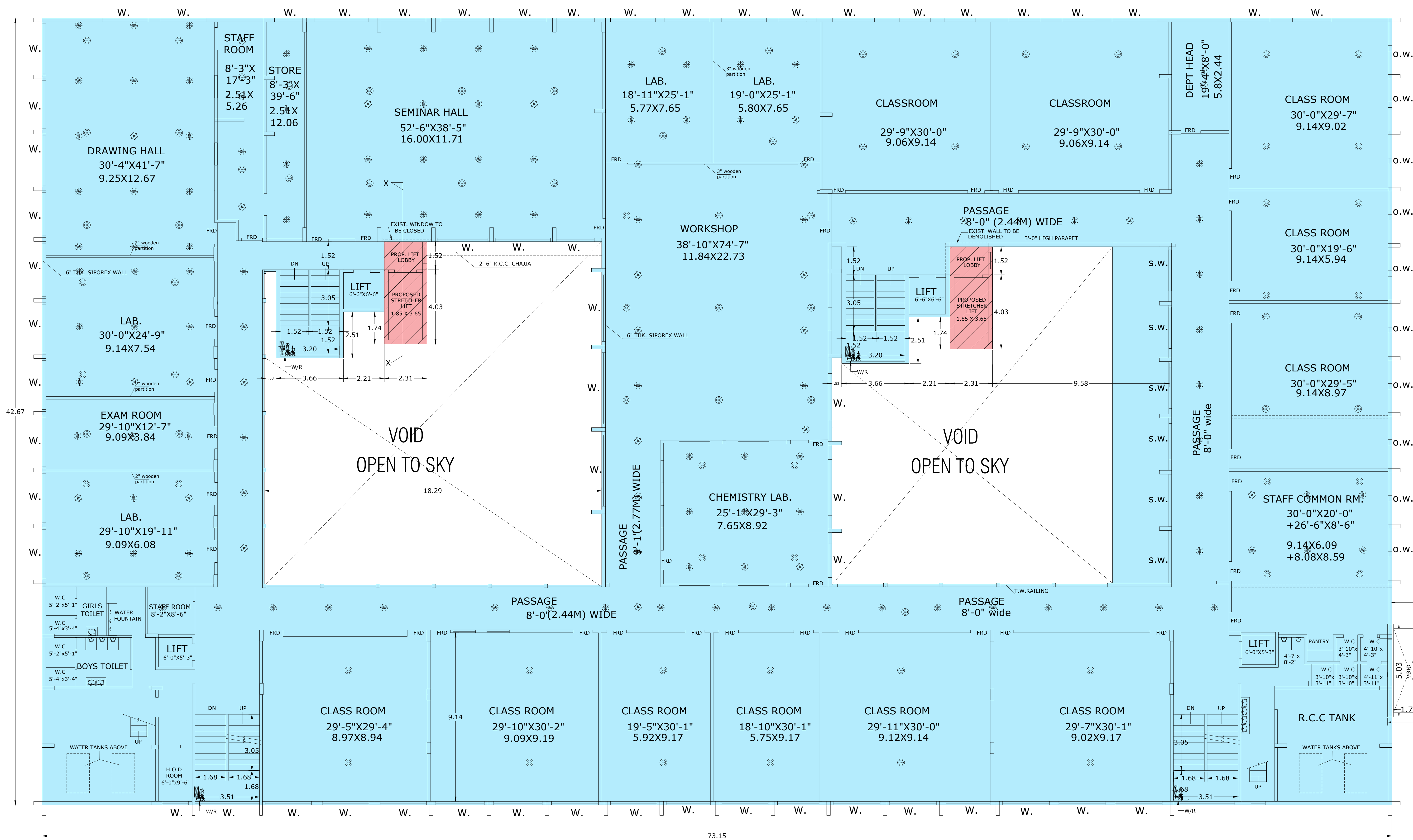
EXISTING FIFTH FLOOR PLAN SCALE : 1:100
