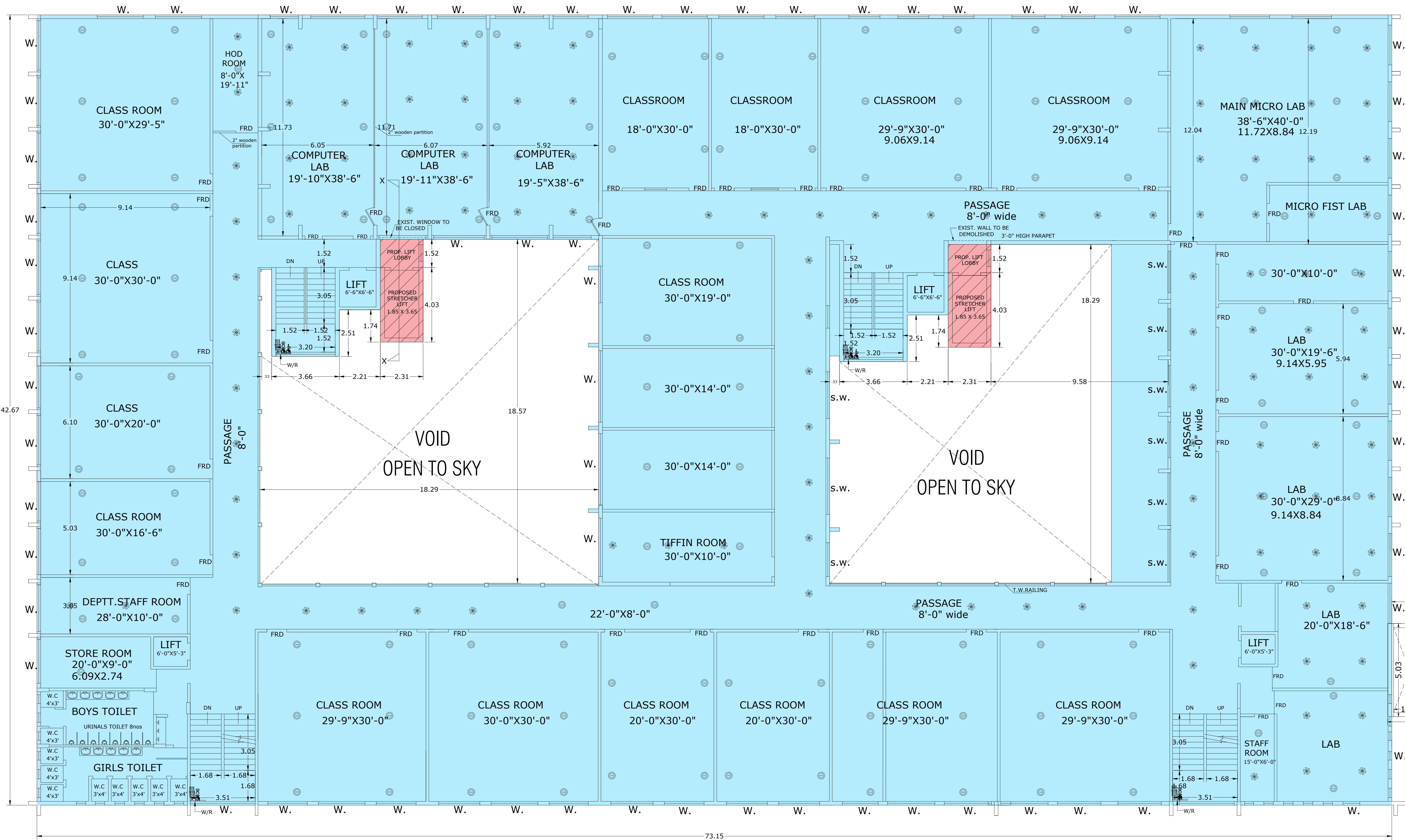
EXISTING THIRD FLOOR PLAN SCALE : 1:100
