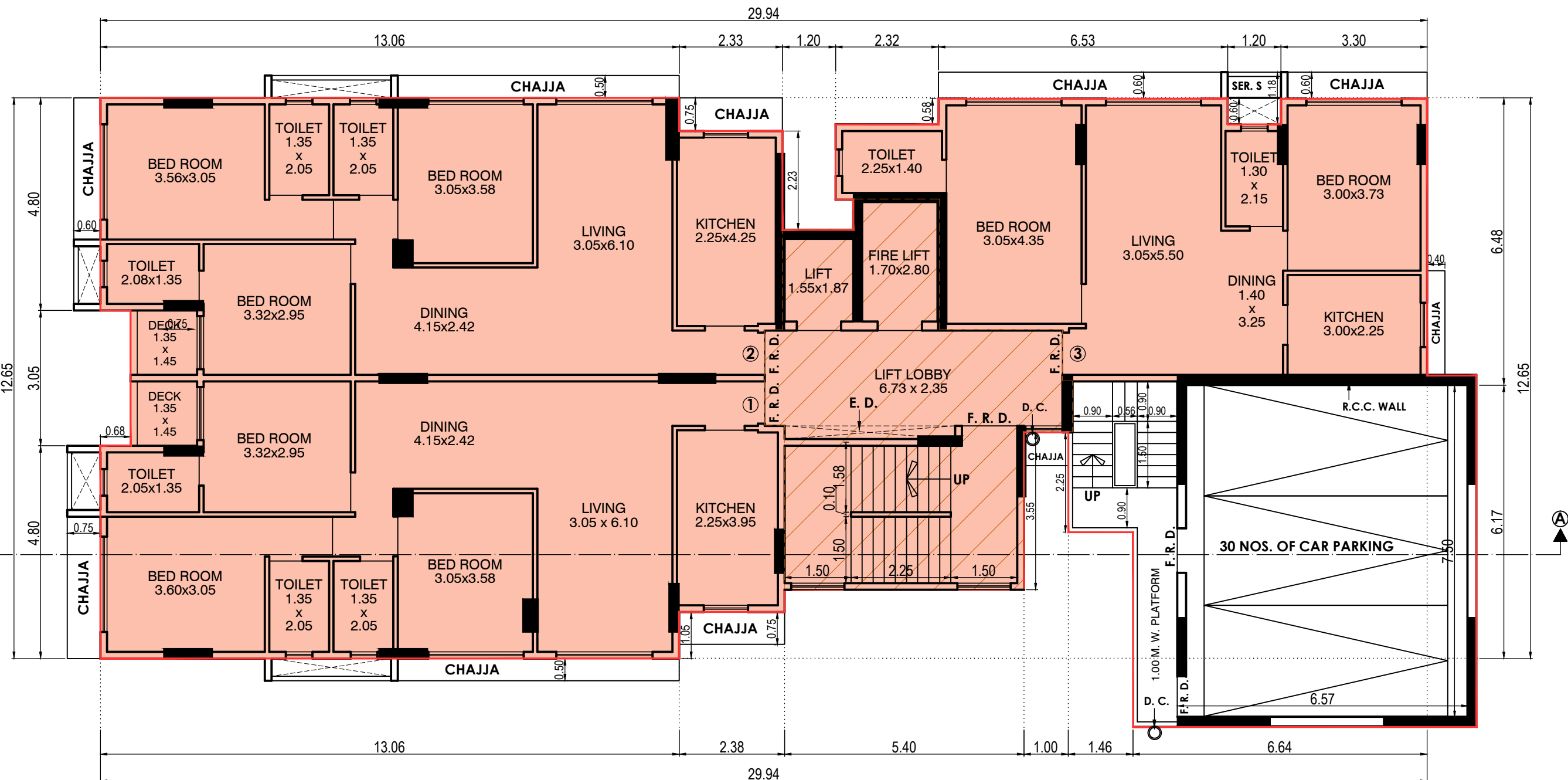
7TH & 8TH FLOOR PLAN SCALE :- 1:100
