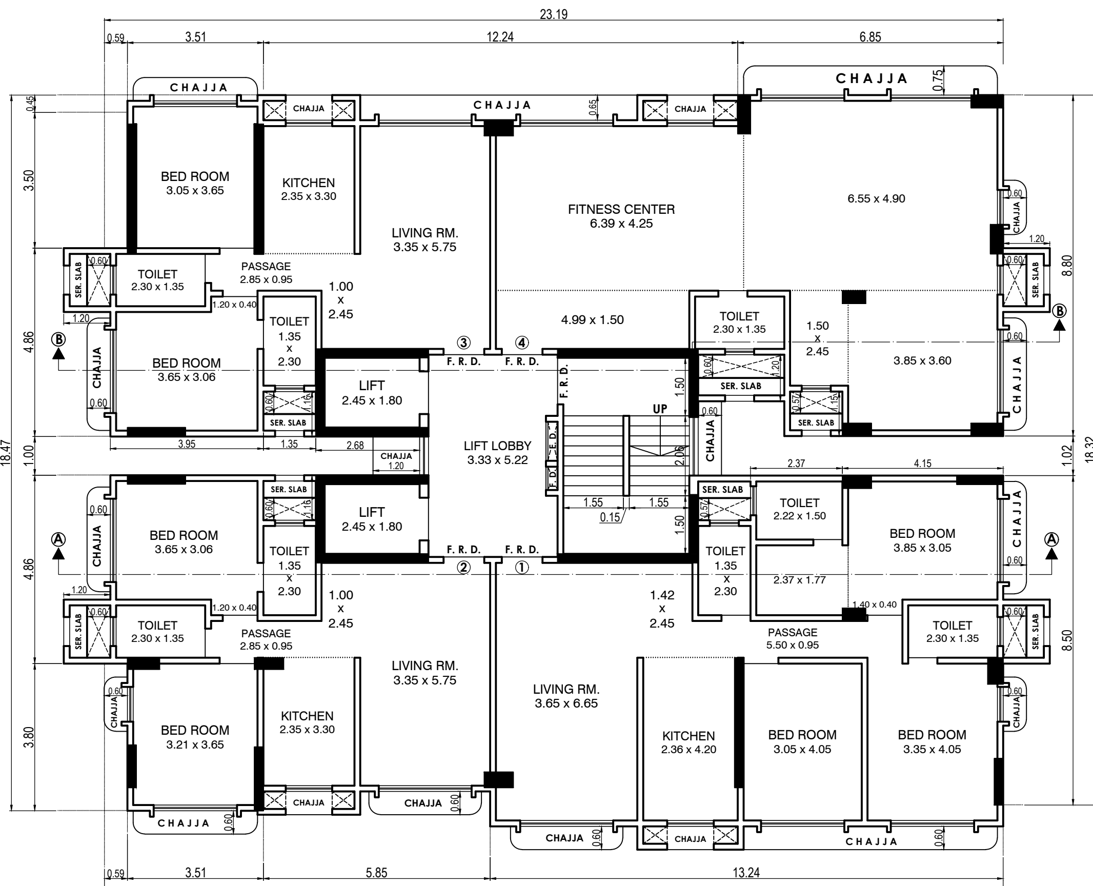
16TH FLOOR PLAN SCALE :- 1:100
