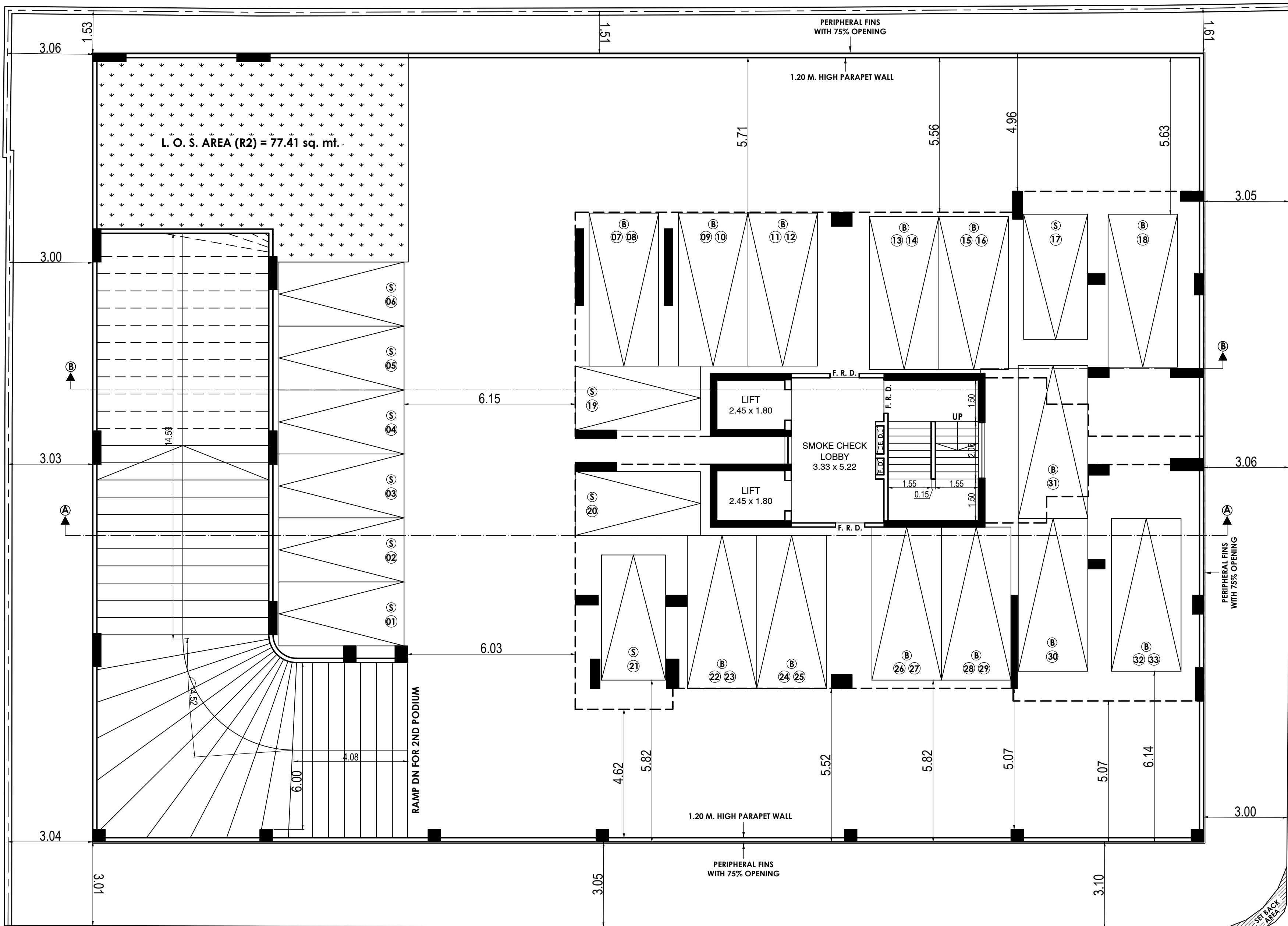
3RD PODIUM FLOOR PLAN SCALE :- 1:100
