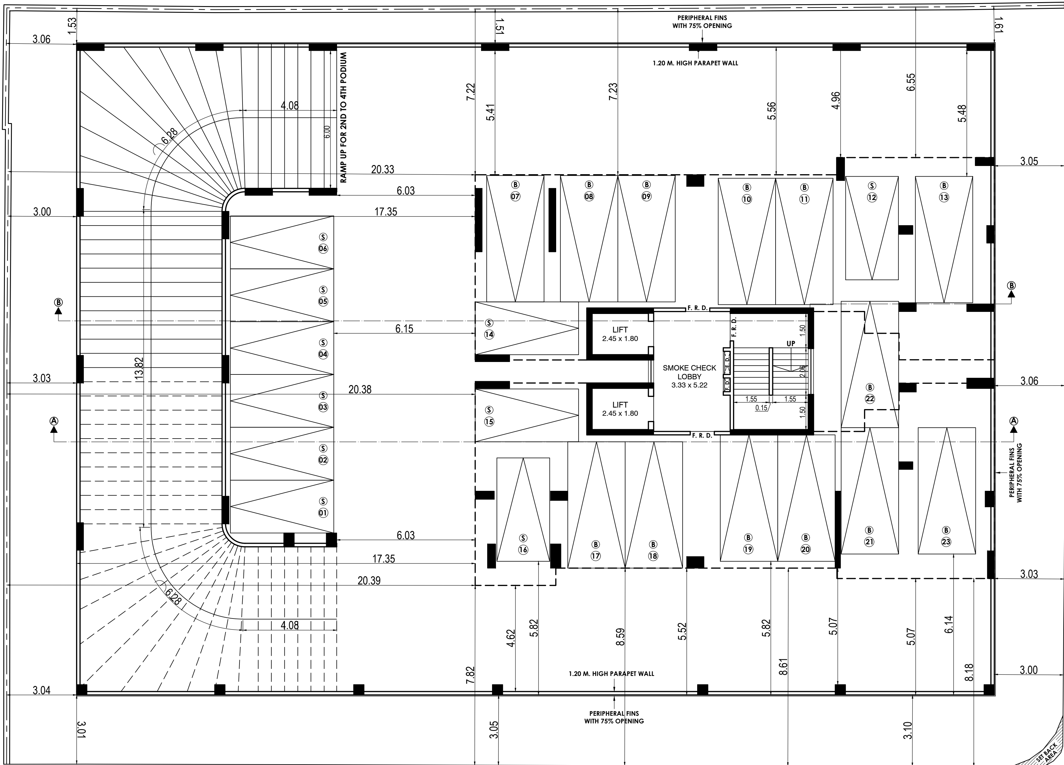
1ST & 2ND PODIUM FLOOR PLAN SCALE :- 1:100
