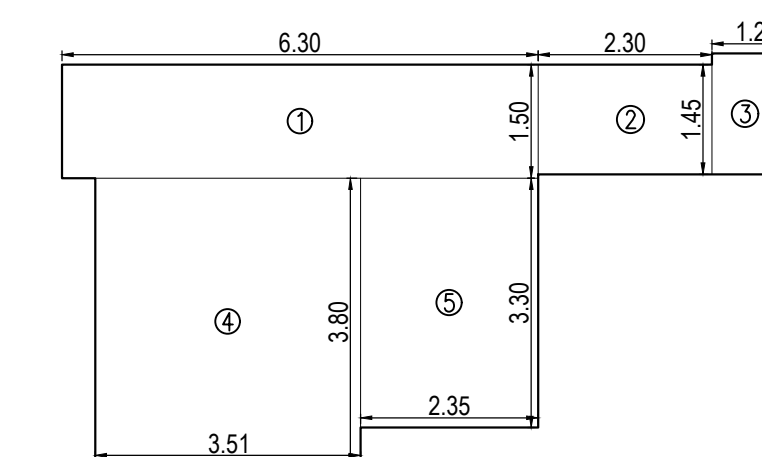
REFUGE AREA LINE DIAGRAM (14TH FLOOR) SCALE :- 1:100
