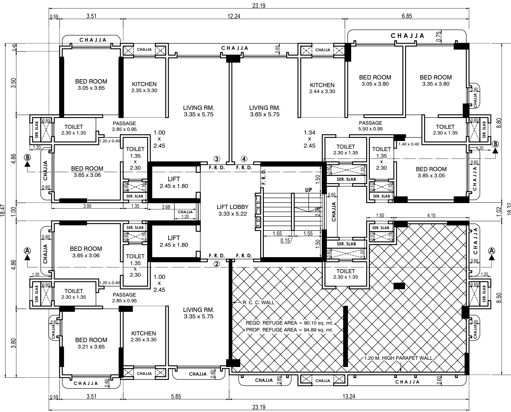
7TH FLOOR PLAN SCALE :- 1:100
