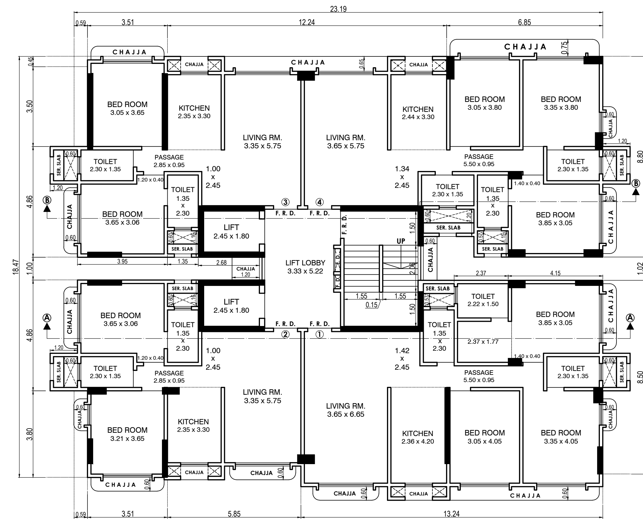
10TH TO 13TH & 15TH FLOOR PLAN SCALE :- 1:100
