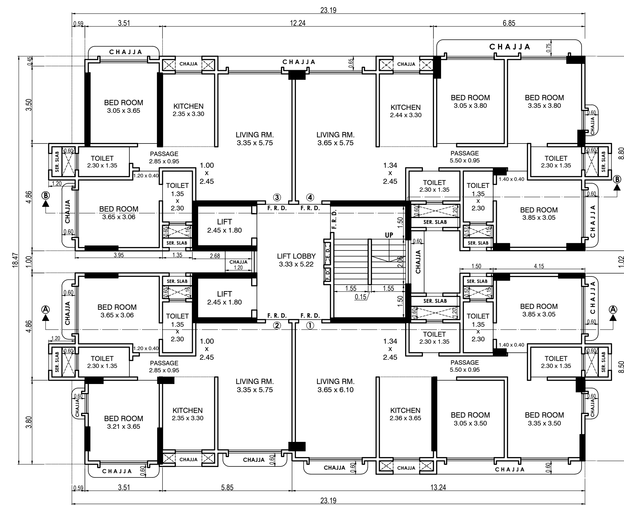
8TH & 9TH FLOOR PLAN SCALE :- 1:100
