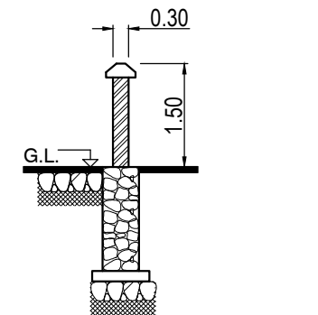
SECTION THRO' COMPOUND WALL
