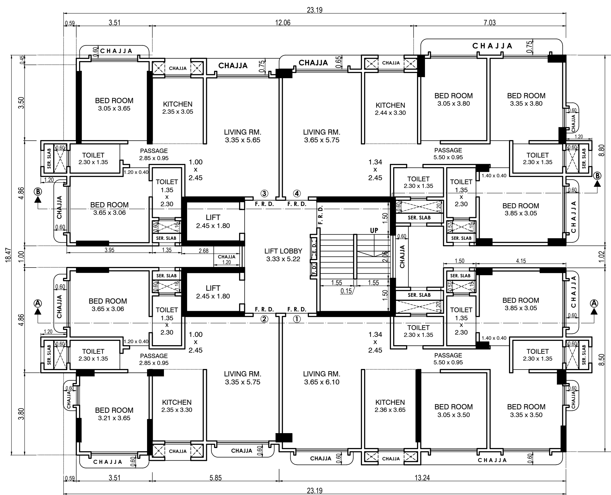
5TH & 6TH FLOOR PLAN SCALE :- 1:100
