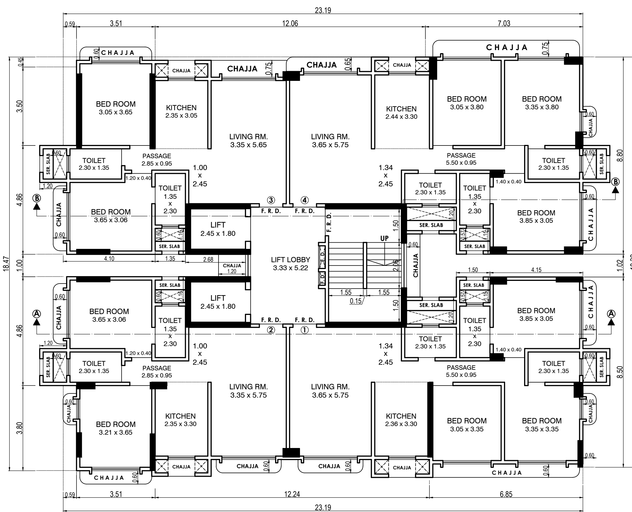
4TH FLOOR PLAN SCALE :- 1:100
