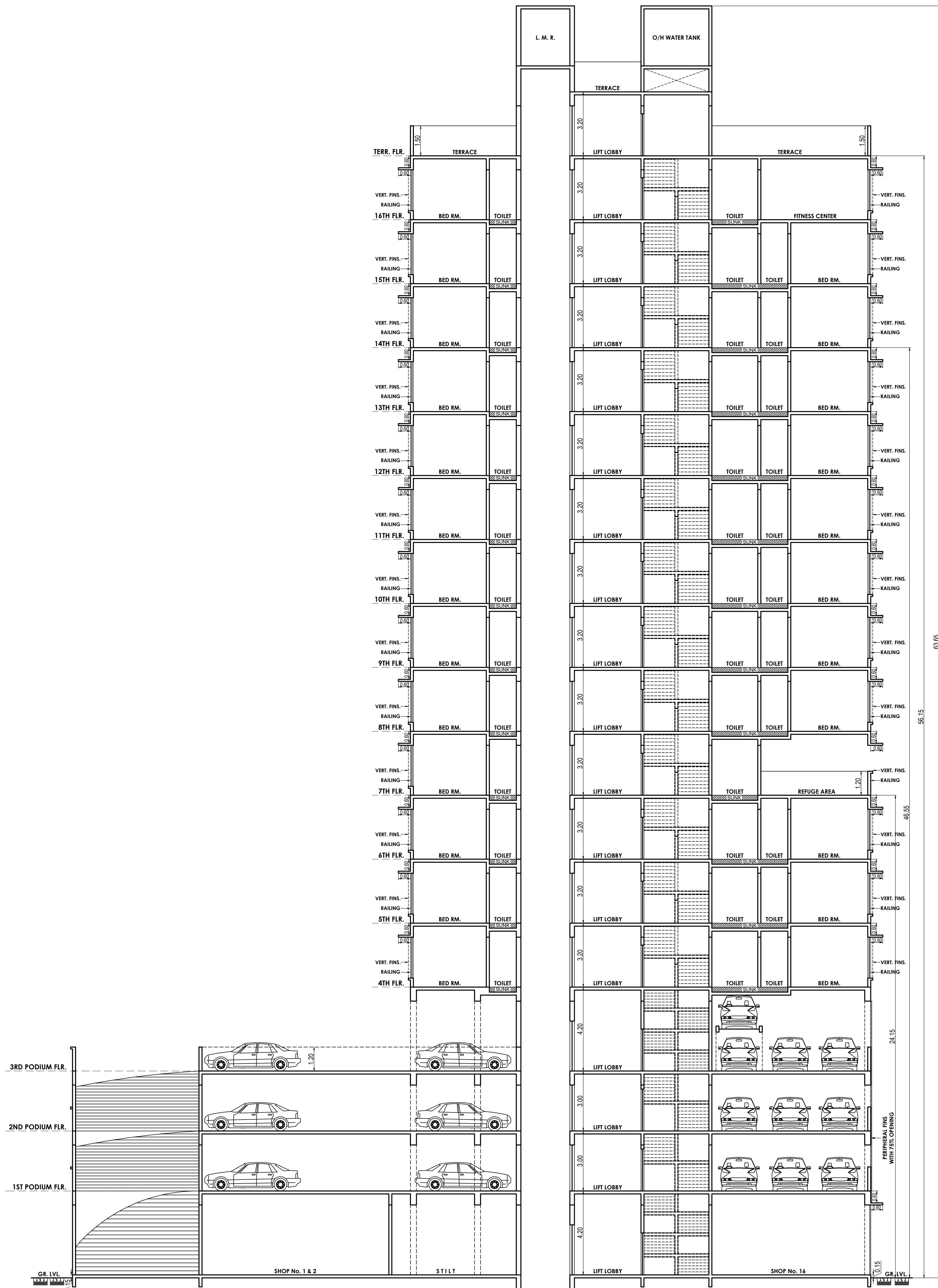
SECTION B - B SCALE :- 1:100
