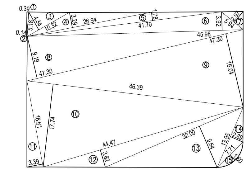
PLOT AREA LINE DIAGRAM
