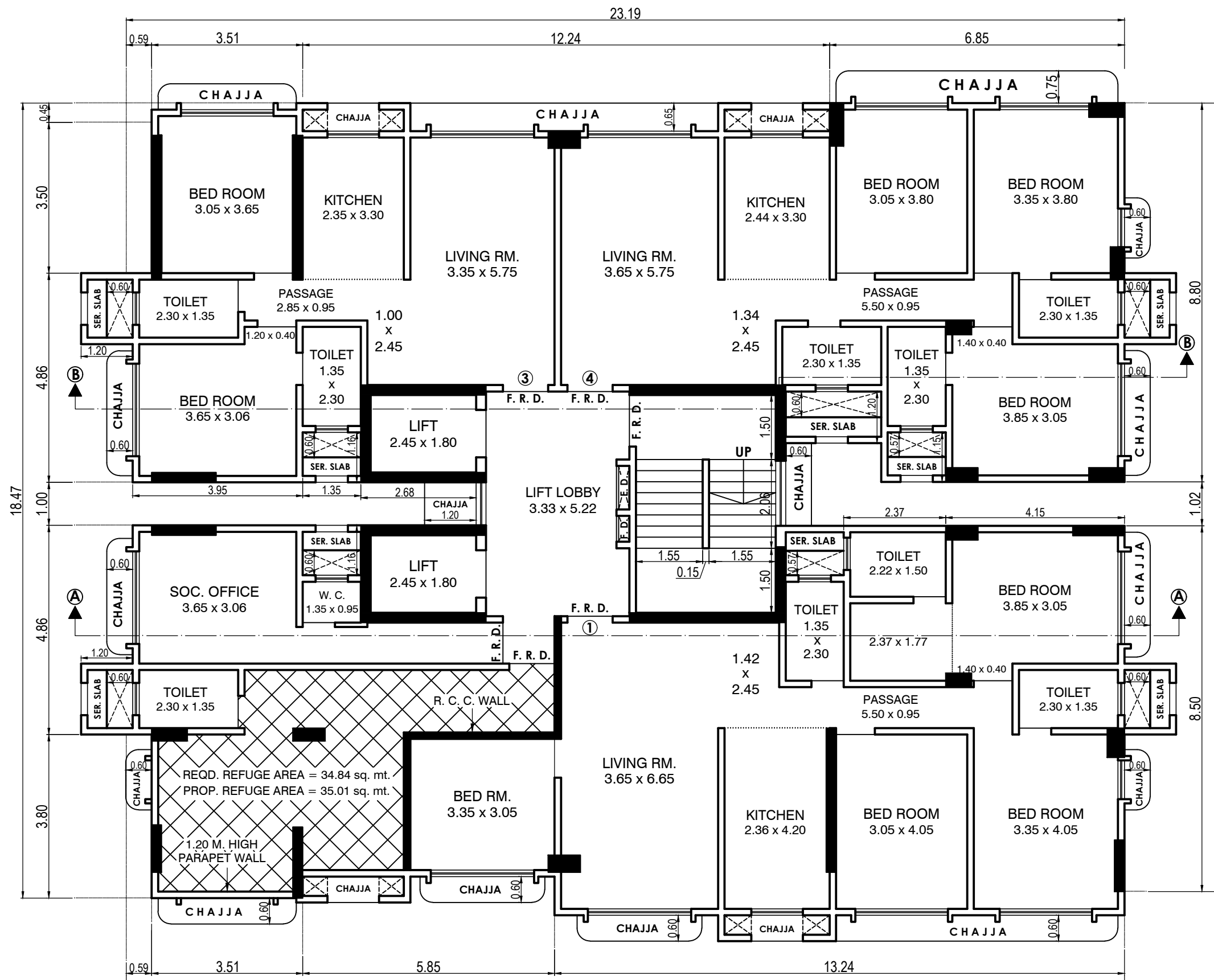
14TH FLOOR PLAN SCALE :- 1:100
