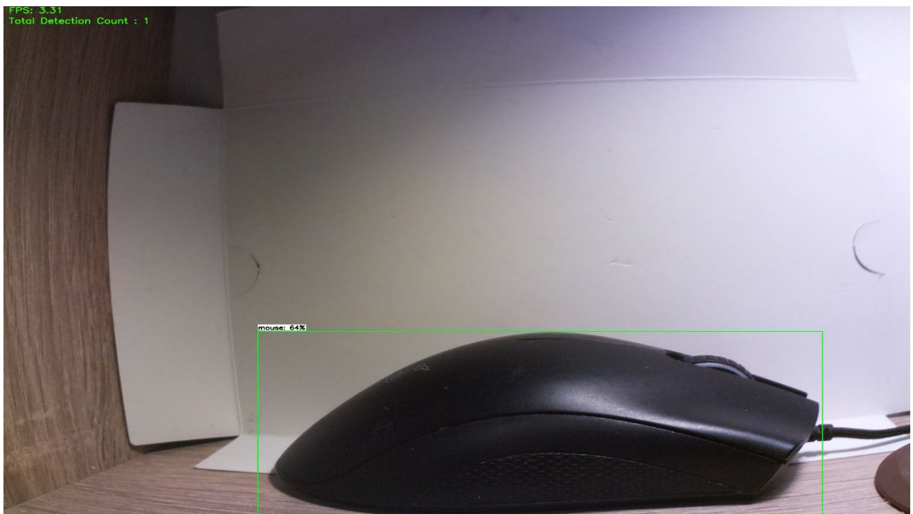
Figure 3: Object Detection
