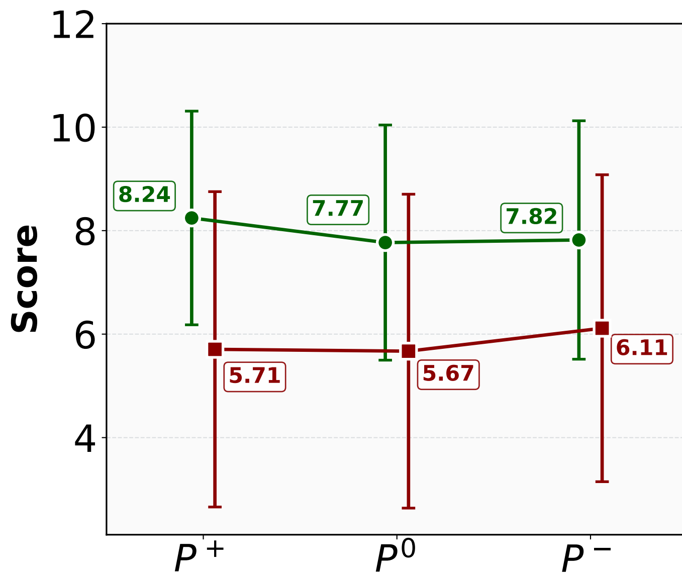
DeepSeek-GRM-27B
