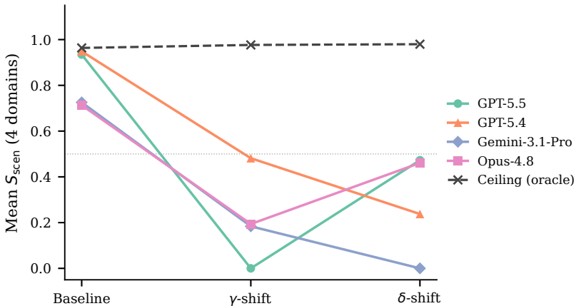
Frontier LLMs cliff-drop on \gamma/\delta shifts
