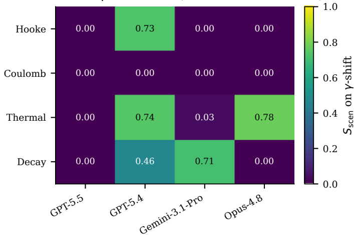
Per-domain \gamma -shift score (4 domains \times 4 models)
