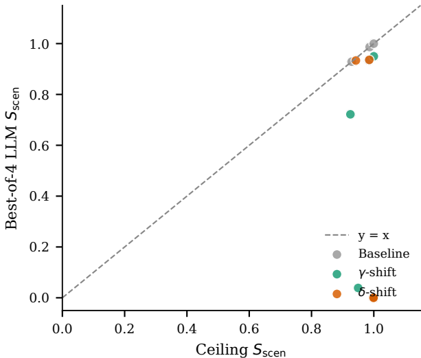
Ceiling vs. best LLM (12 cells)
