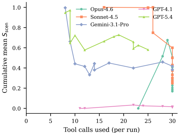
Tool-call efficiency (cumulative)
