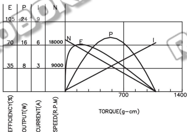
Base Motor Characteristic Graph
