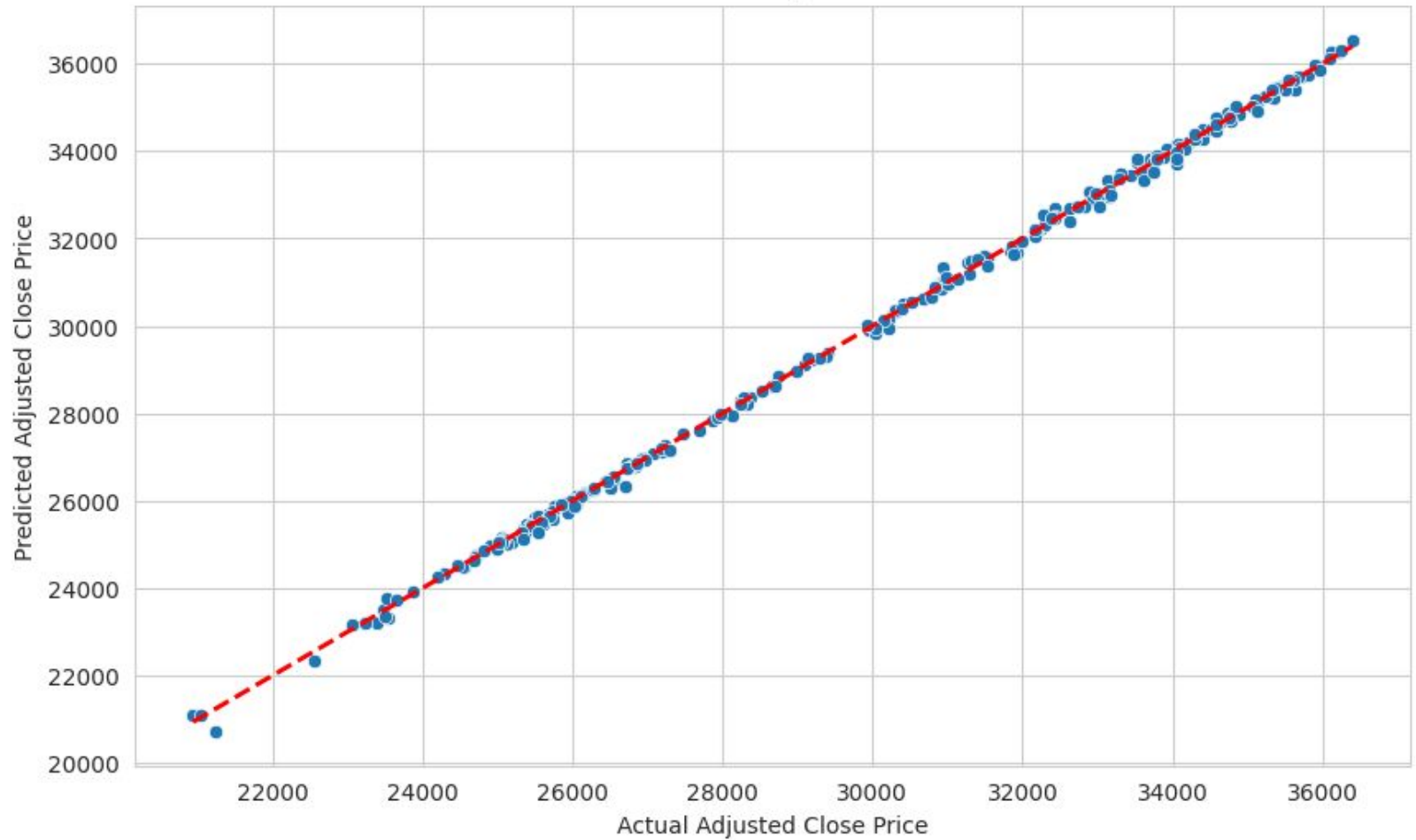
Actual vs Predicted Adjusted Close Prices
