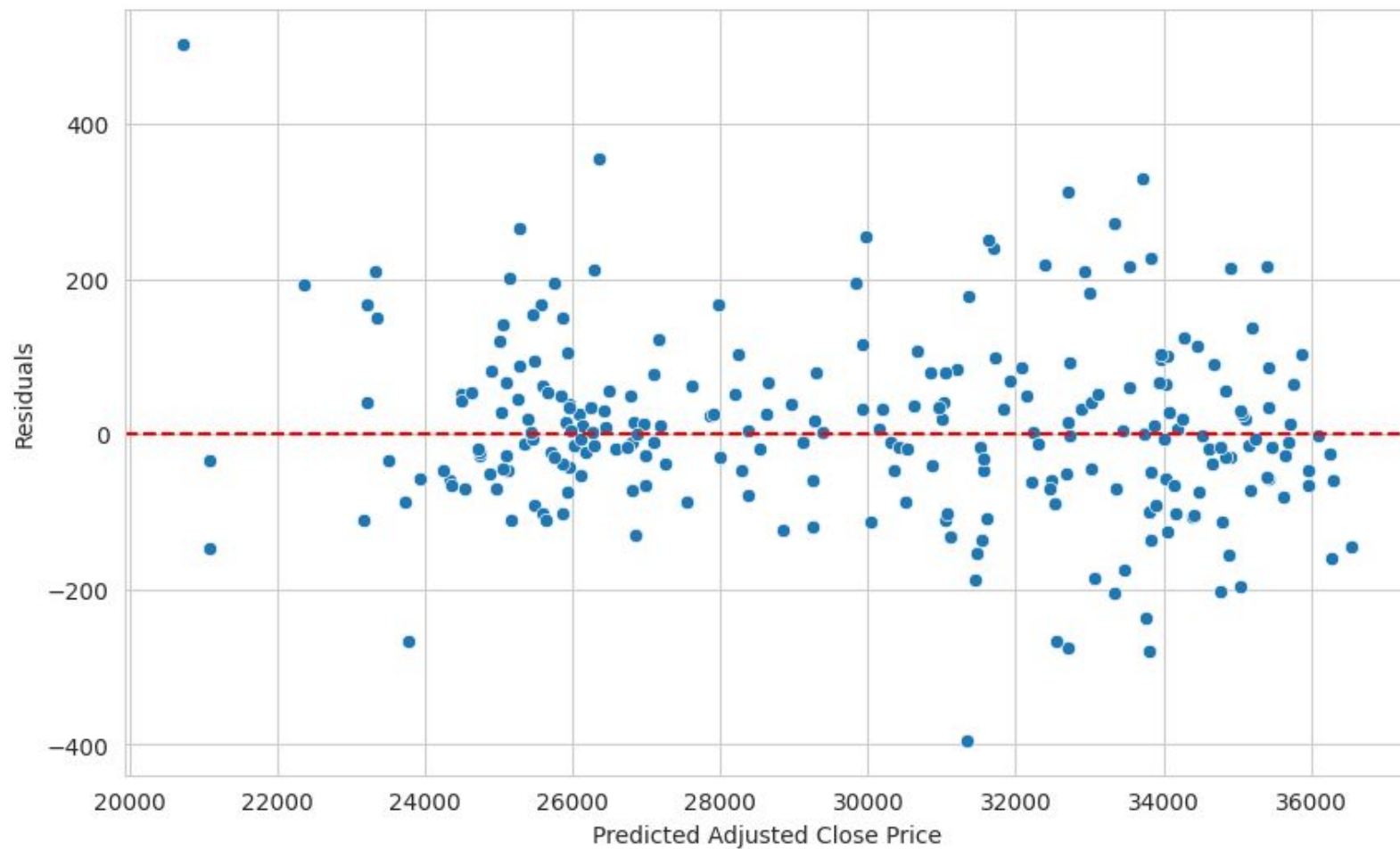
Residuals vs Predicted Values
