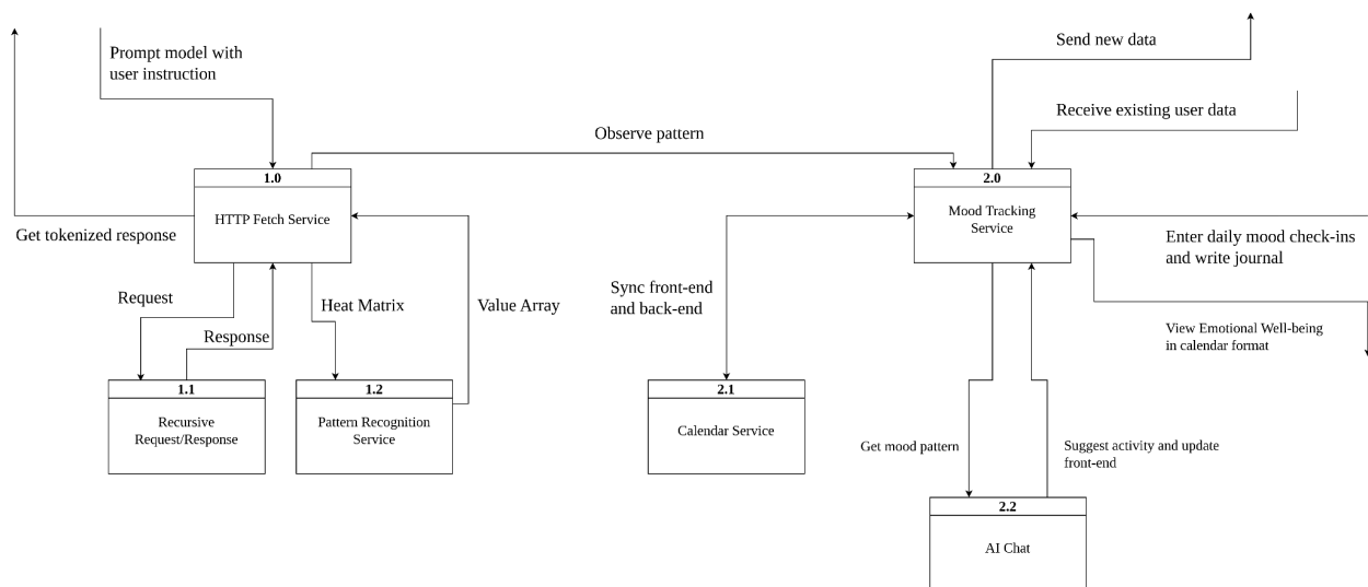
Figure: Level 2 Data Flow Diagram.
