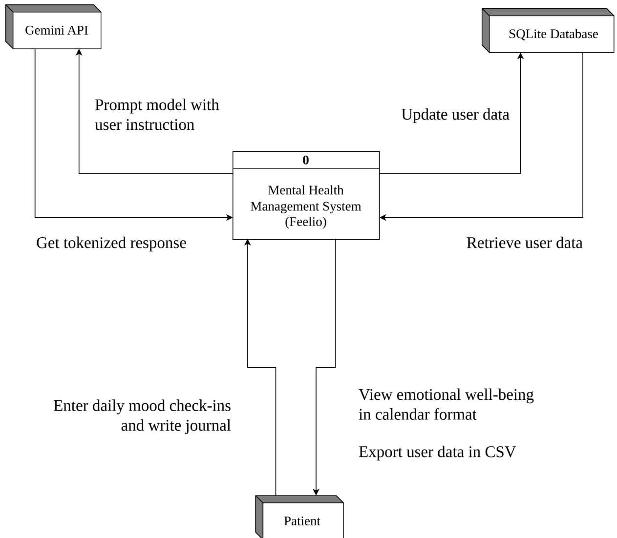
Figure: Context Level (Level 0) Data Flow Diagram.
