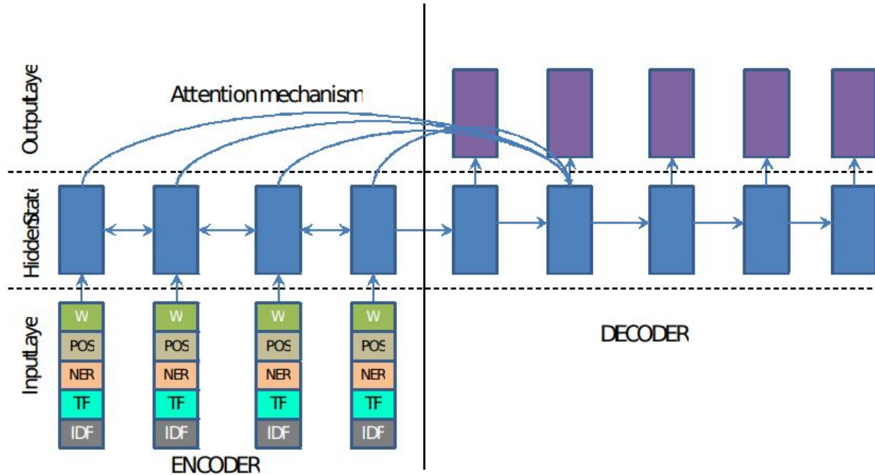
Typical Encoder-Attend-Decoder architecture.
