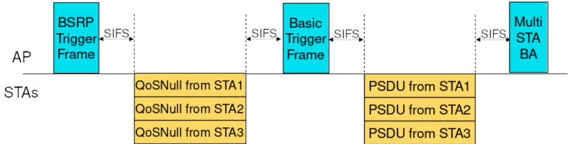
Frame exchange sequences using UL OFDMA
