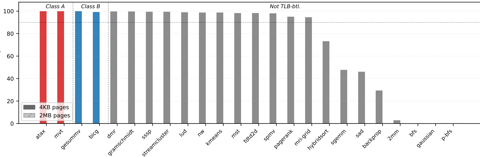
L2 TLB Dead-Entry Ratio (%)
