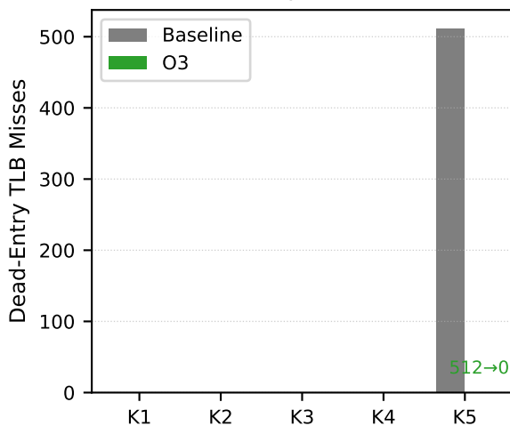
Dead-Entry Miss Count
