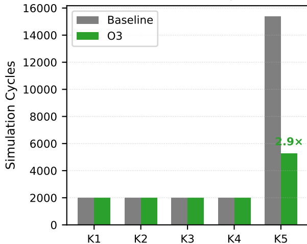
Kernel Execution Cycles
