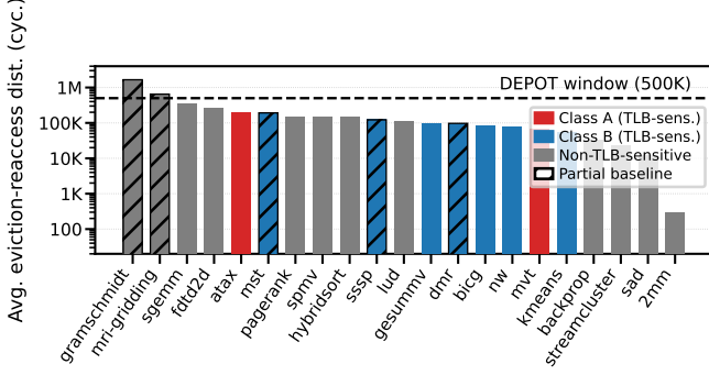
Figure 4: Average eviction-to-reaccess distance (log scale) per workload vs. DEPOT’s default protection window, for all 21 workloads with measurable dead-entry activity. Hatched bars are from partially-converged baselines.
