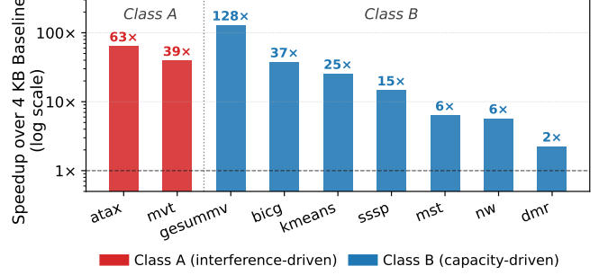
Figure 5: IPC speedup under 2 MB pages over 4 KB baseline for all 9 TLB-sensitive workloads.
