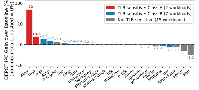
Figure 7: IPC improvement of DEPOT over 4 KB baseline for all 24 workloads, sorted descending.
