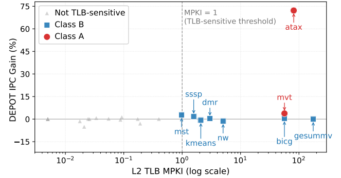
Figure 8: IPC improvement of DEPOT vs. L2 TLB MPKI for all 24 workloads.
