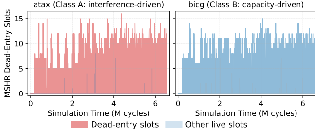
Figure 4: MSHR dead-slot occupancy over time for atax and bicg .
