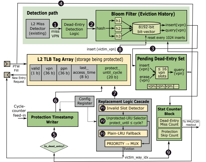
Figure 6: DEPOT mechanism: eviction-history Bloom filter, Pending Dead-Entry Set, per-entry protection timer, and protection-aware replacement cascade.
